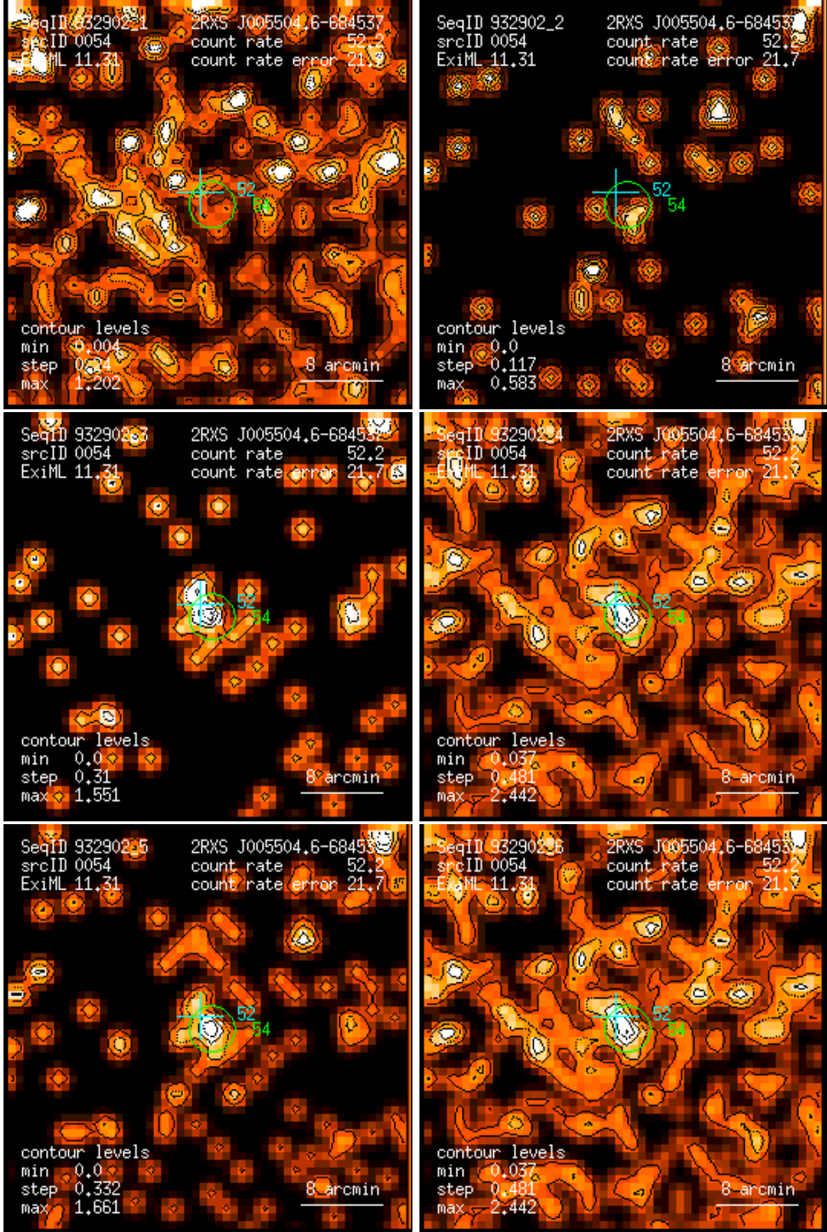
Figure 54: RASS 932902: detection 0054: band rate images, Gaussian filter: (1) PSPC channels 11 – 41, (2) 52 – 90, (3) 91 – 201, (4) 11 – 235, (5) 52 – 201, (6) 11 – 201. Broad band rates in counts/ks. Band rate contour levels in counts/ks/arcmin 2 .
