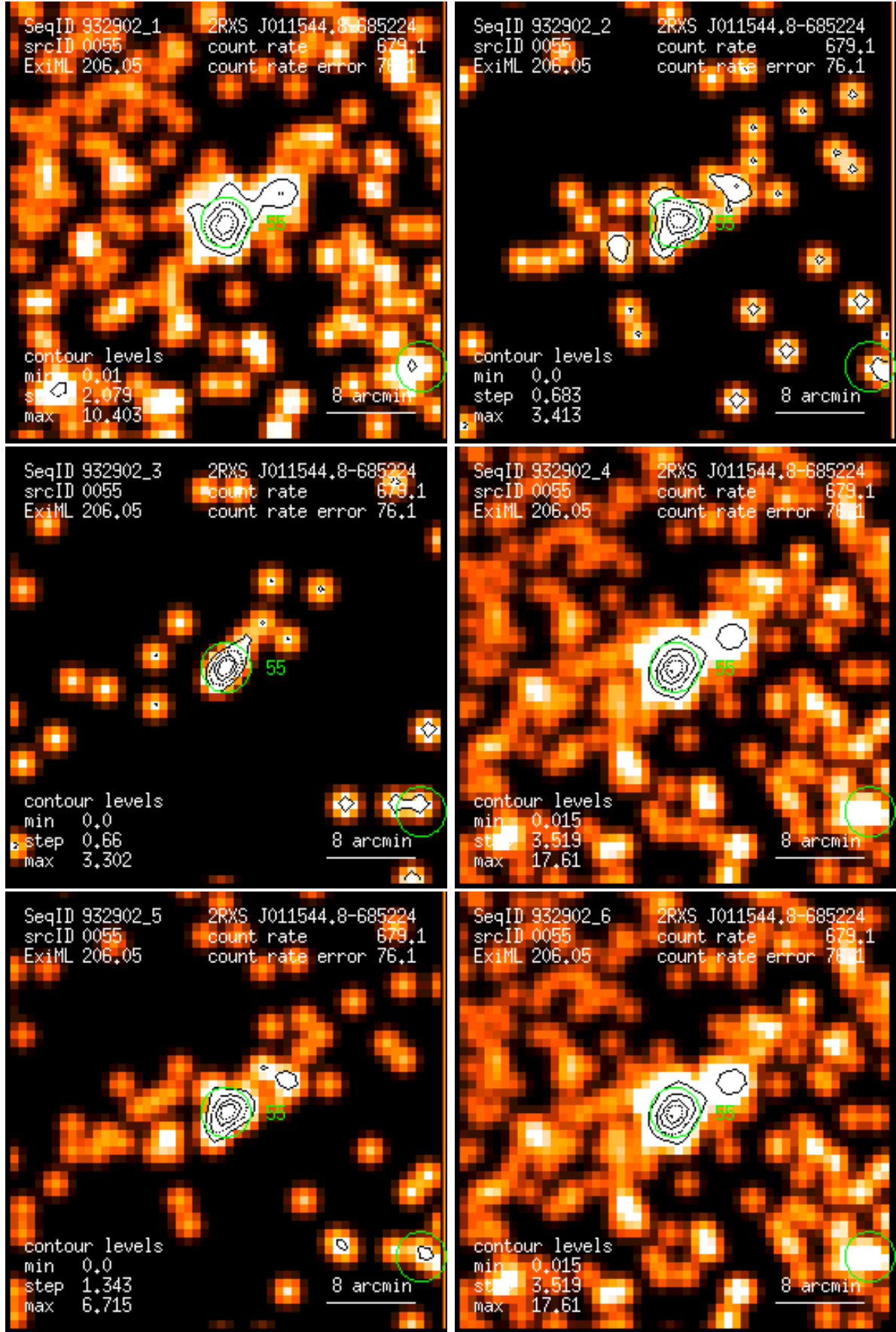
Figure 55: RASS 932902: detection 0055: band rate images, Gaussian filter: (1) PSPC channels 11 – 41, (2) 52 – 90, (3) 91 – 201, (4) 11 – 235, (5) 52 – 201, (6) 11 – 201. Broad band rates in counts/ks. Band rate contour levels in counts/ks/arcmin 2 .
