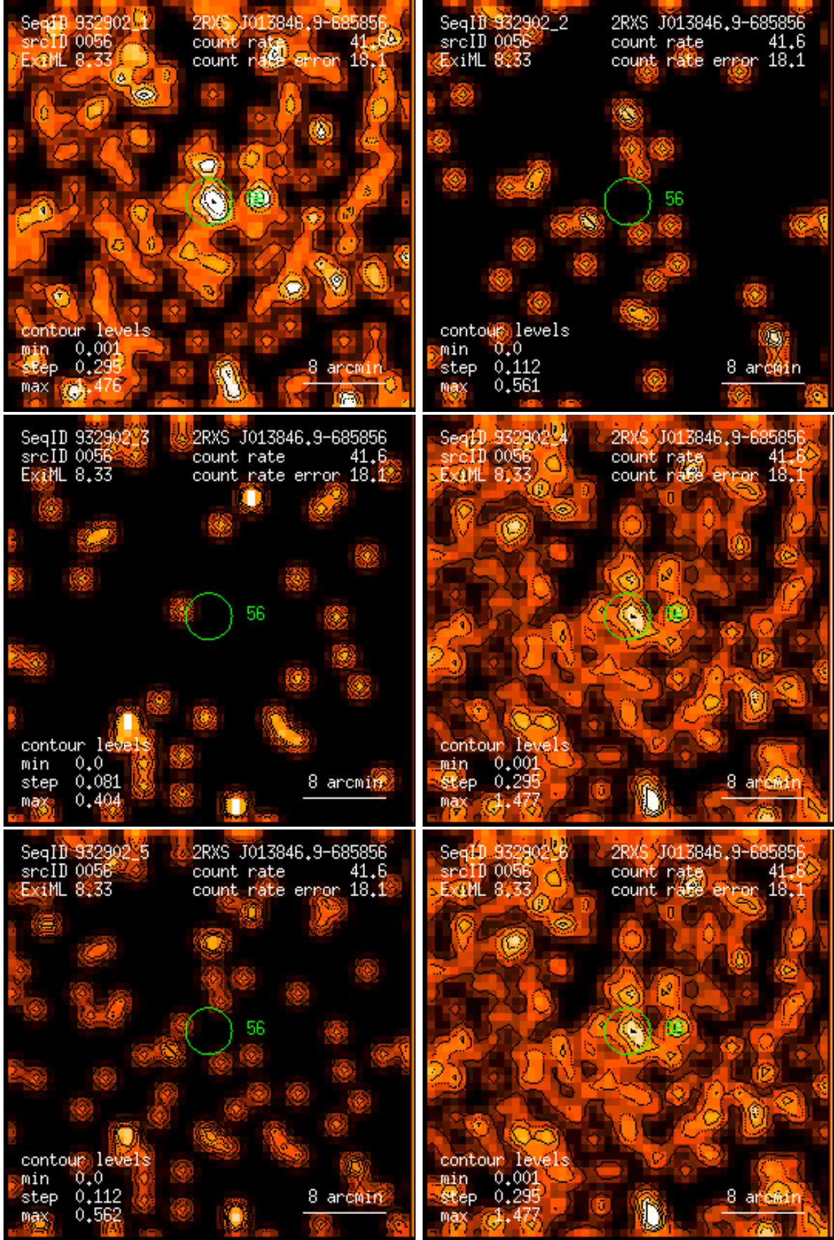
Figure 56: RASS 932902: detection 0056: band rate images, Gaussian filter: (1) PSPC channels 11 – 41, (2) 52 – 90, (3) 91 – 201, (4) 11 – 235, (5) 52 – 201, (6) 11 – 201. Broad band rates in counts/ks. Band rate contour levels in counts/ks/arcmin 2 .
