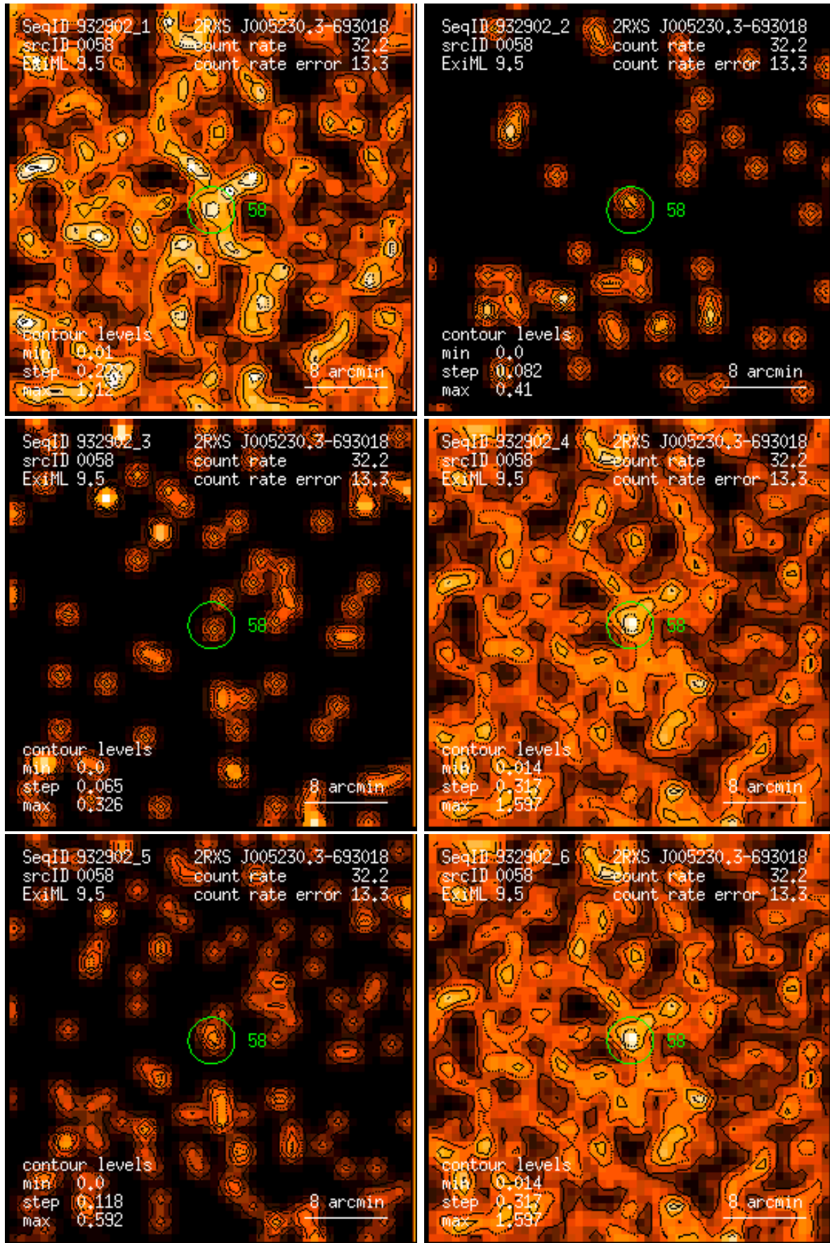
Figure 58: RASS 932902: detection 0058: band rate images, Gaussian filter: (1) PSPC channels 11 – 41, (2) 52 – 90, (3) 91 – 201, (4) 11 – 235, (5) 52 – 201, (6) 11 – 201. Broad band rates in counts/ks. Band rate contour levels in counts/ks/arcmin 2 .
