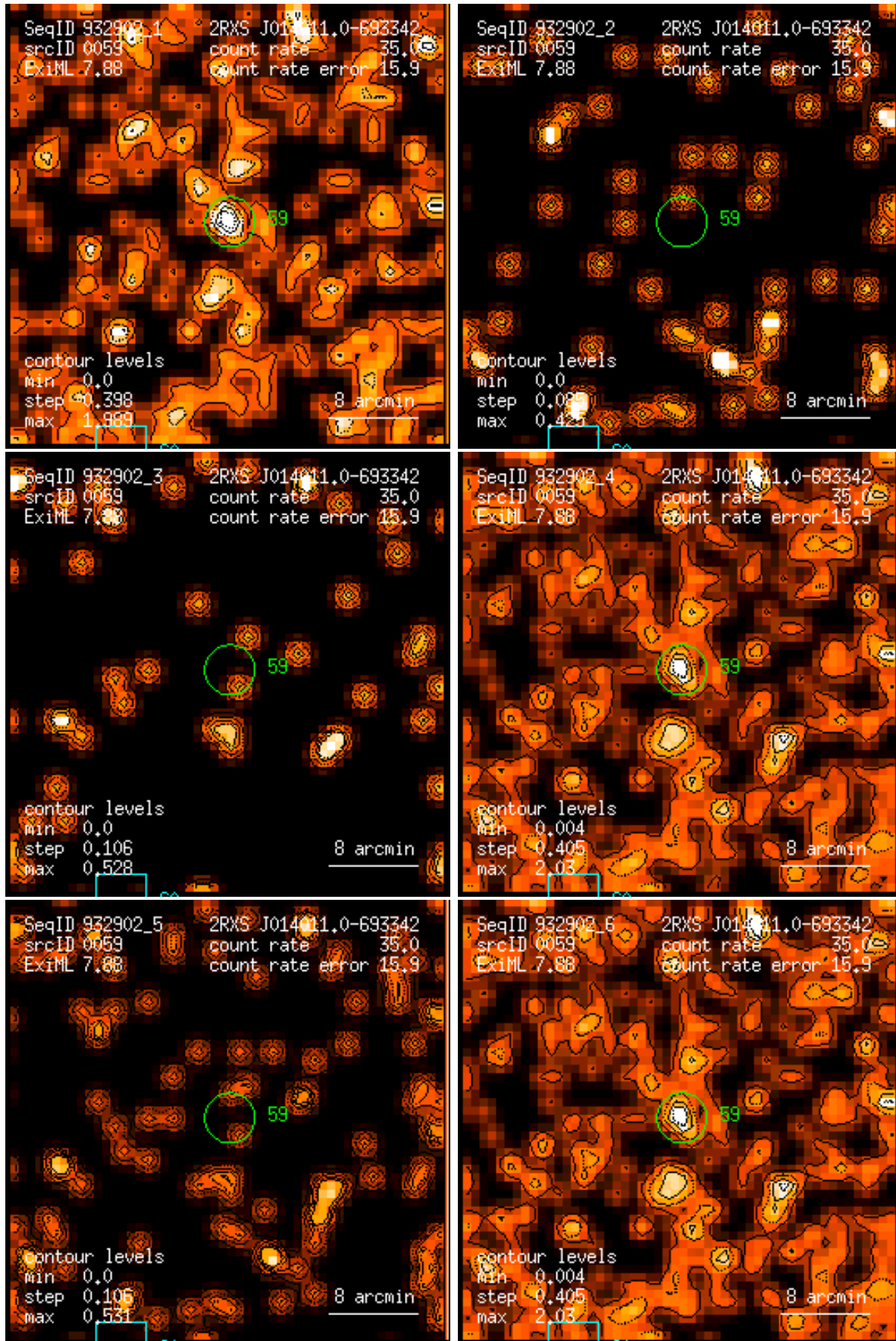
Figure 59: RASS 932902: detection 0059: band rate images, Gaussian filter: (1) PSPC channels 11 – 41, (2) 52 – 90, (3) 91 – 201, (4) 11 – 235, (5) 52 – 201, (6) 11 – 201. Broad band rates in counts/ks. Band rate contour levels in counts/ks/arcmin 2 .
