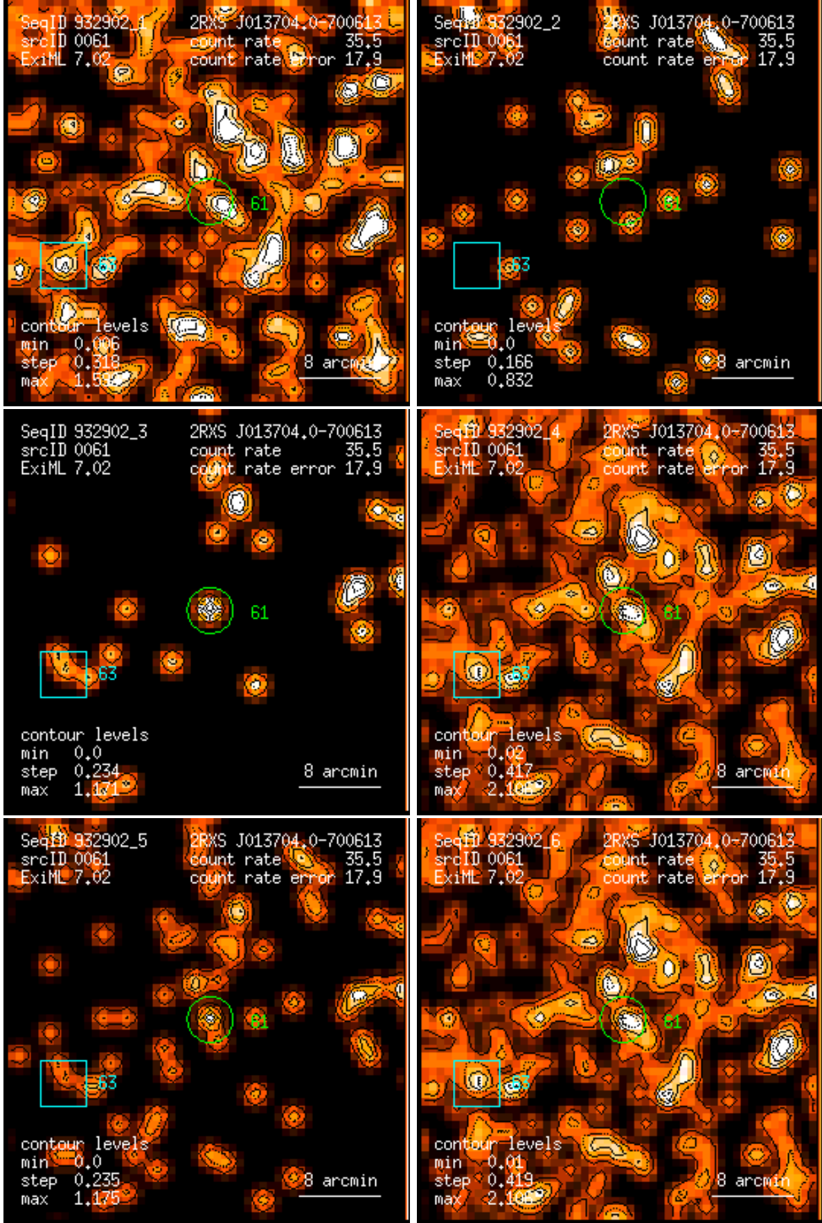
Figure 61: RASS 932902: detection 0061: band rate images, Gaussian filter: (1) PSPC channels 11 – 41, (2) 52 – 90, (3) 91 – 201, (4) 11 – 235, (5) 52 – 201, (6) 11 – 201. Broad band rates in counts/ks. Band rate contour levels in counts/ks/arcmin 2 .
