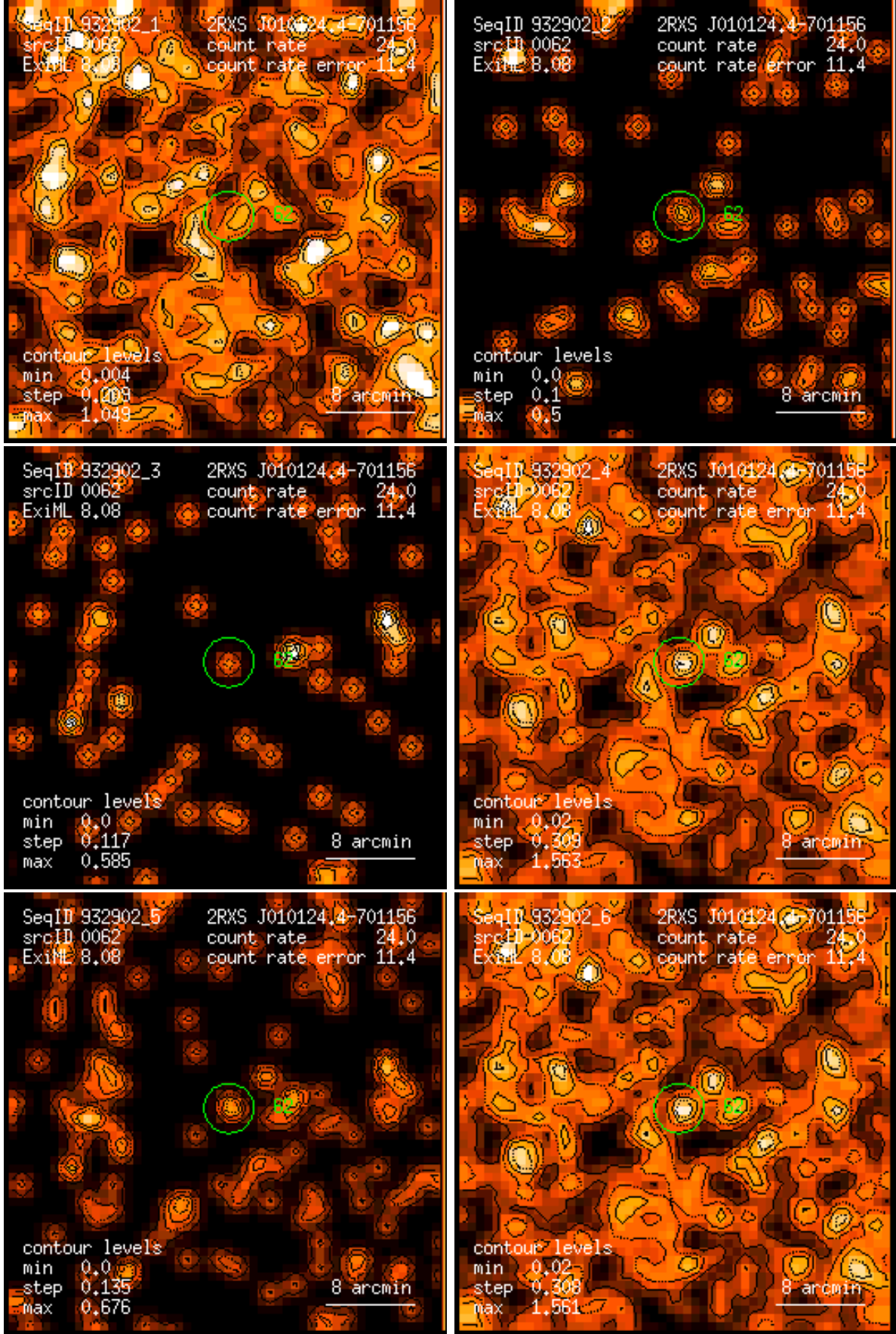
Figure 62: RASS 932902: detection 0062: band rate images, Gaussian filter: (1) PSPC channels 11 – 41, (2) 52 – 90, (3) 91 – 201, (4) 11 – 235, (5) 52 – 201, (6) 11 – 201. Broad band rates in counts/ks. Band rate contour levels in counts/ks/arcmin 2 .
