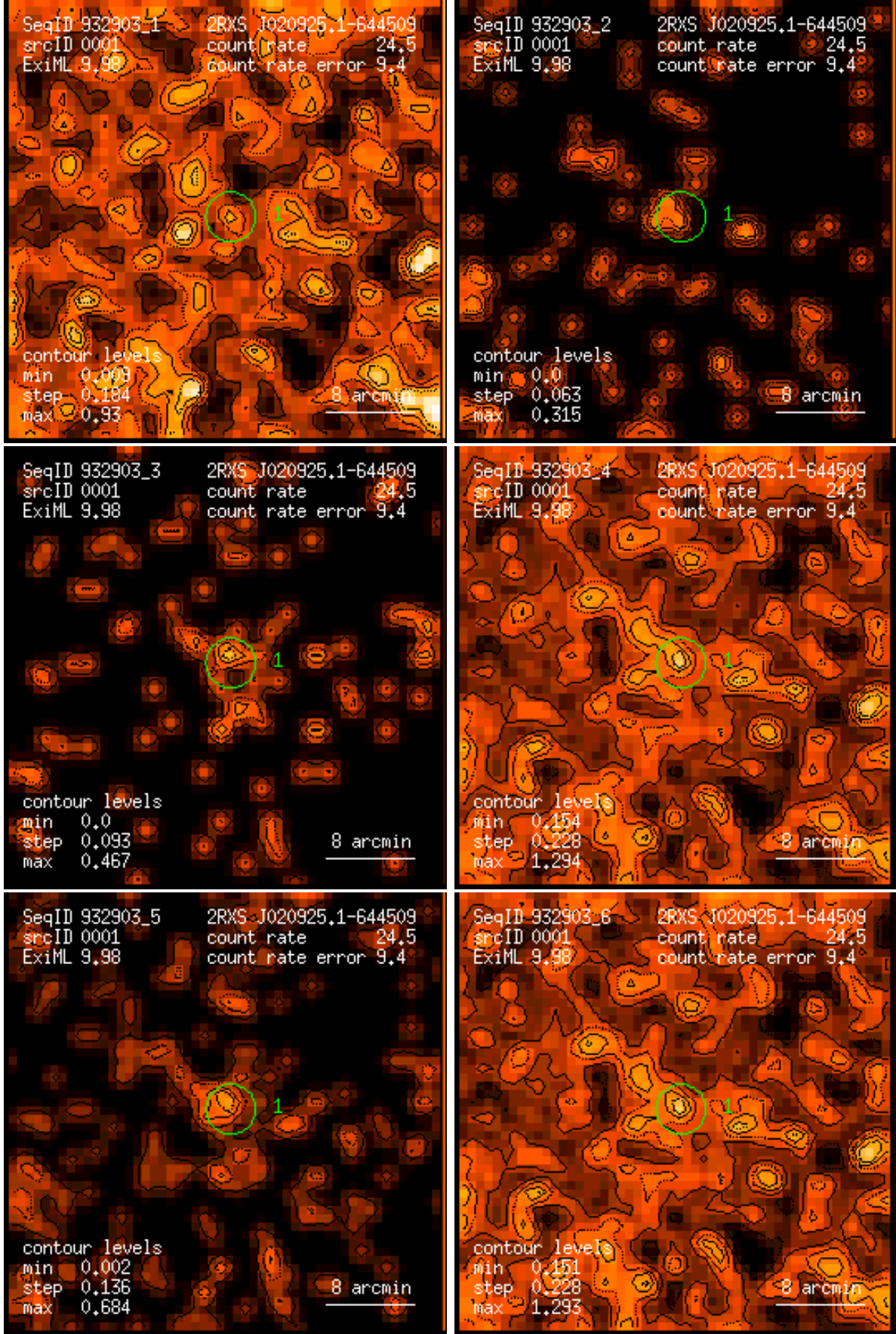
Figure 1: RASS 932903: detection 0001: band rate images, Gaussian filter: (1) PSPC channels 11 – 41, (2) 52 – 90, (3) 91 – 201, (4) 11 – 235, (5) 52 – 201, (6) 11 – 201. Broad band rates in counts/ks. Band rate contour levels in counts/ks/arcmin 2 .
