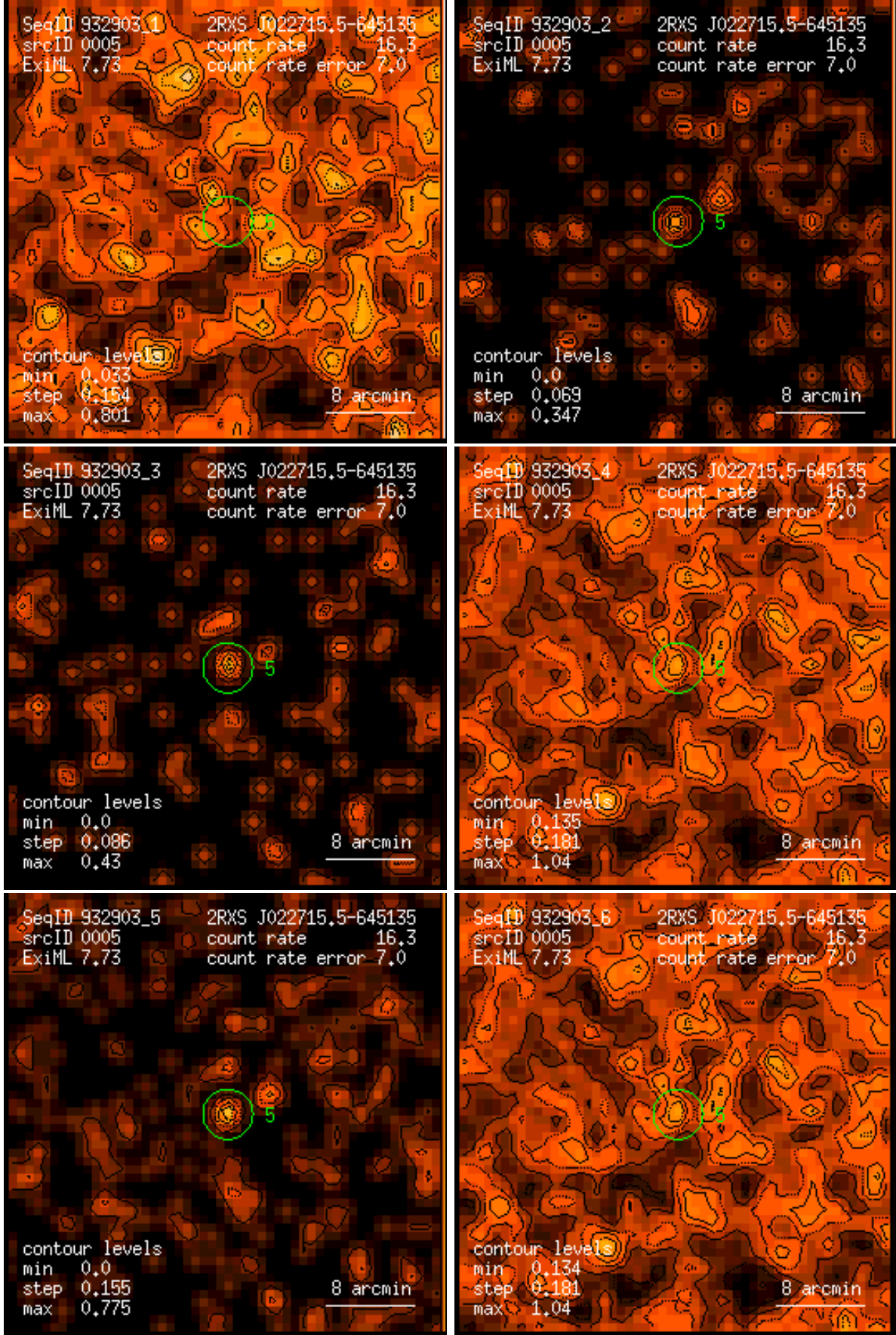
Figure 5: RASS 932903: detection 0005: band rate images, Gaussian filter: (1) PSPC channels 11 – 41, (2) 52 – 90, (3) 91 – 201, (4) 11 – 235, (5) 52 – 201, (6) 11 – 201. Broad band rates in counts/ks. Band rate contour levels in counts/ks/arcmin 2 .
