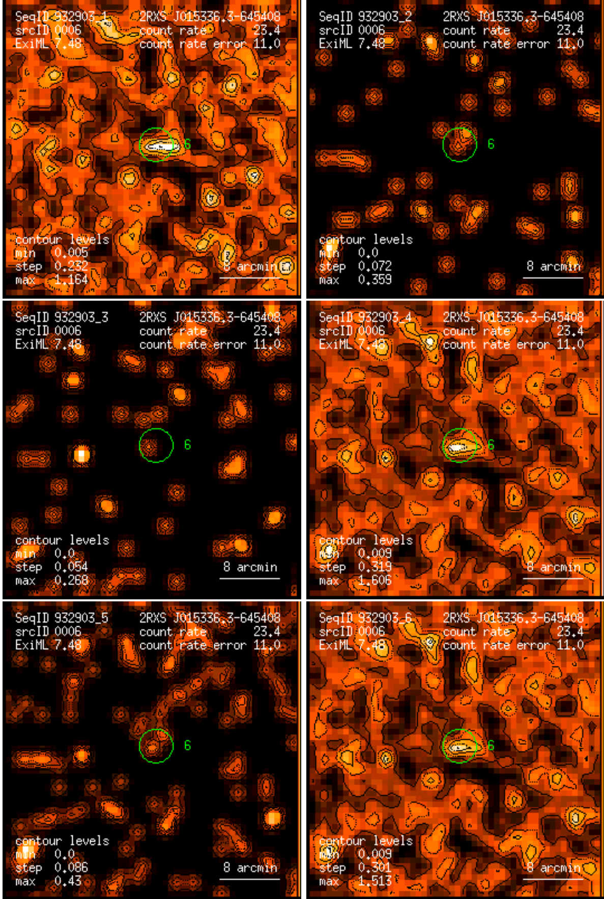
Figure 6: RASS 932903: detection 0006: band rate images, Gaussian filter: (1) PSPC channels 11 – 41, (2) 52 – 90, (3) 91 – 201, (4) 11 – 235, (5) 52 – 201, (6) 11 – 201. Broad band rates in counts/ks. Band rate contour levels in counts/ks/arcmin 2 .
