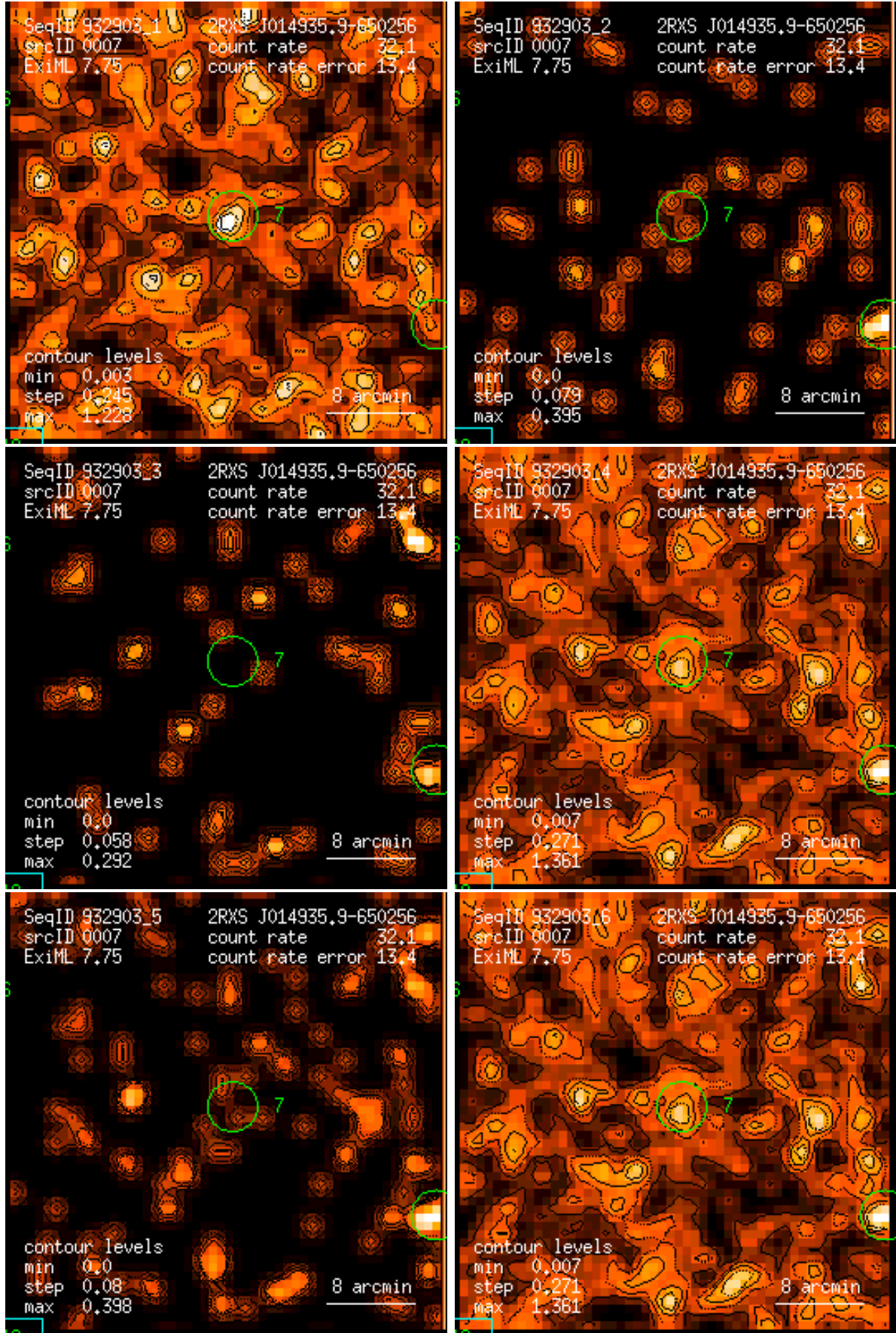
Figure 7: RASS 932903: detection 0007: band rate images, Gaussian filter: (1) PSPC channels 11 – 41, (2) 52 – 90, (3) 91 – 201, (4) 11 – 235, (5) 52 – 201, (6) 11 – 201. Broad band rates in counts/ks. Band rate contour levels in counts/ks/arcmin 2 .
