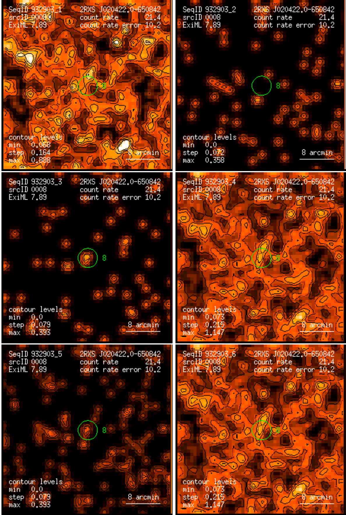
Figure 8: RASS 932903: detection 0008: band rate images, Gaussian filter: (1) PSPC channels 11 – 41, (2) 52 – 90, (3) 91 – 201, (4) 11 – 235, (5) 52 – 201, (6) 11 – 201. Broad band rates in counts/ks. Band rate contour levels in counts/ks/arcmin 2 .
