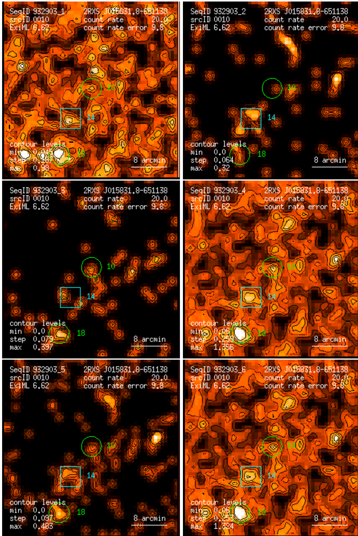
Figure 10: RASS 932903: detection 0010: band rate images, Gaussian filter: (1) PSPC channels 11 – 41, (2) 52 – 90, (3) 91 – 201, (4) 11 – 235, (5) 52 – 201, (6) 11 – 201. Broad band rates in counts/ks. Band rate contour levels in counts/ks/arcmin 2 .
