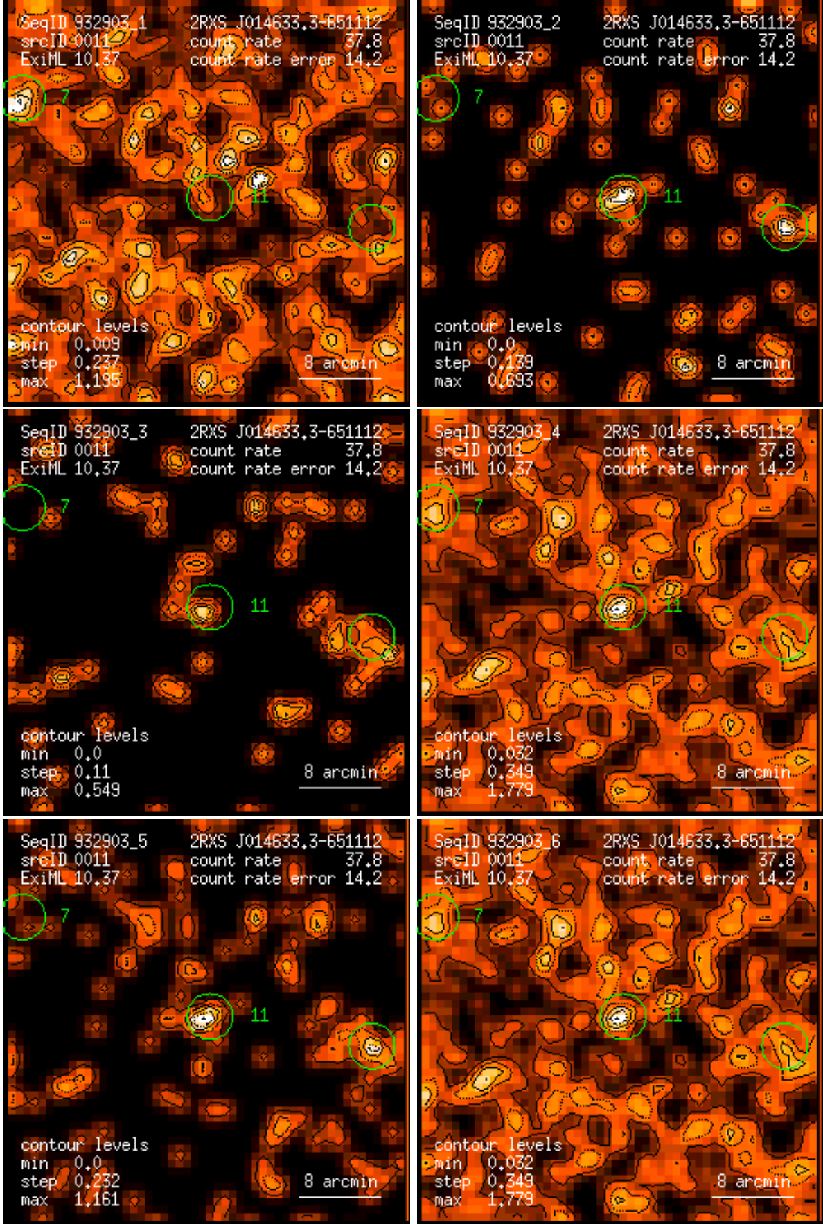
Figure 11: RASS 932903: detection 0011: band rate images, Gaussian filter: (1) PSPC channels 11 – 41, (2) 52 – 90, (3) 91 – 201, (4) 11 – 235, (5) 52 – 201, (6) 11 – 201. Broad band rates in counts/ks. Band rate contour levels in counts/ks/arcmin 2 .
