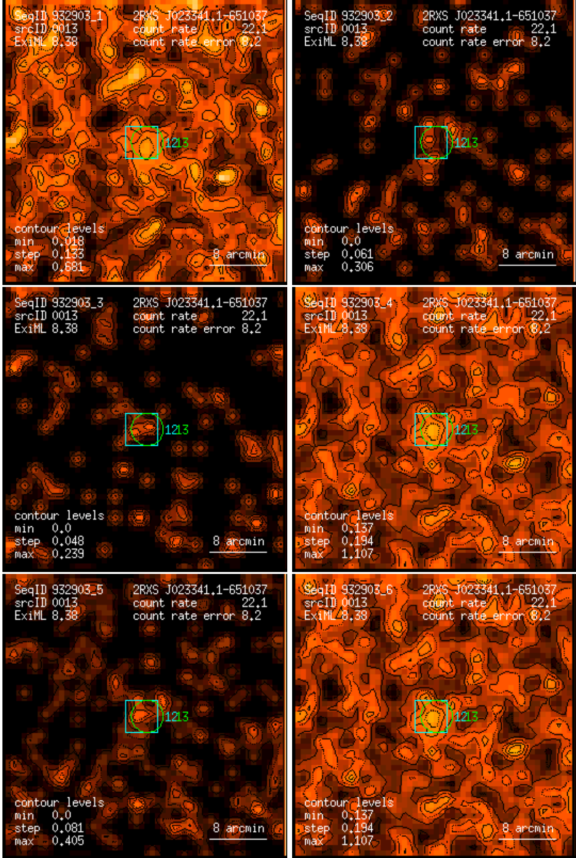
Figure 13: RASS 932903: detection 0013: band rate images, Gaussian filter: (1) PSPC channels 11 – 41, (2) 52 – 90, (3) 91 – 201, (4) 11 – 235, (5) 52 – 201, (6) 11 – 201. Broad band rates in counts/ks. Band rate contour levels in counts/ks/arcmin 2 .
