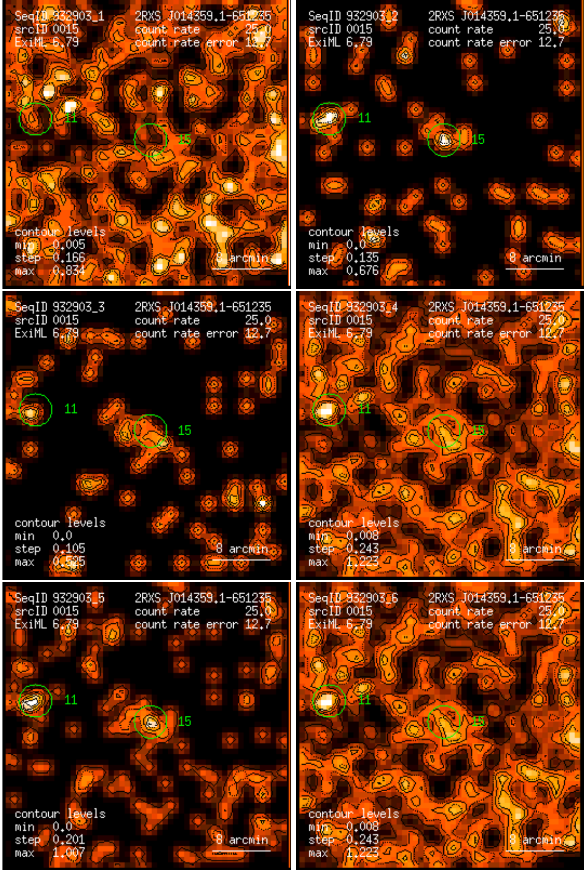
Figure 15: RASS 932903: detection 0015: band rate images, Gaussian filter: (1) PSPC channels 11 – 41, (2) 52 – 90, (3) 91 – 201, (4) 11 – 235, (5) 52 – 201, (6) 11 – 201. Broad band rates in counts/ks. Band rate contour levels in counts/ks/arcmin 2 .
