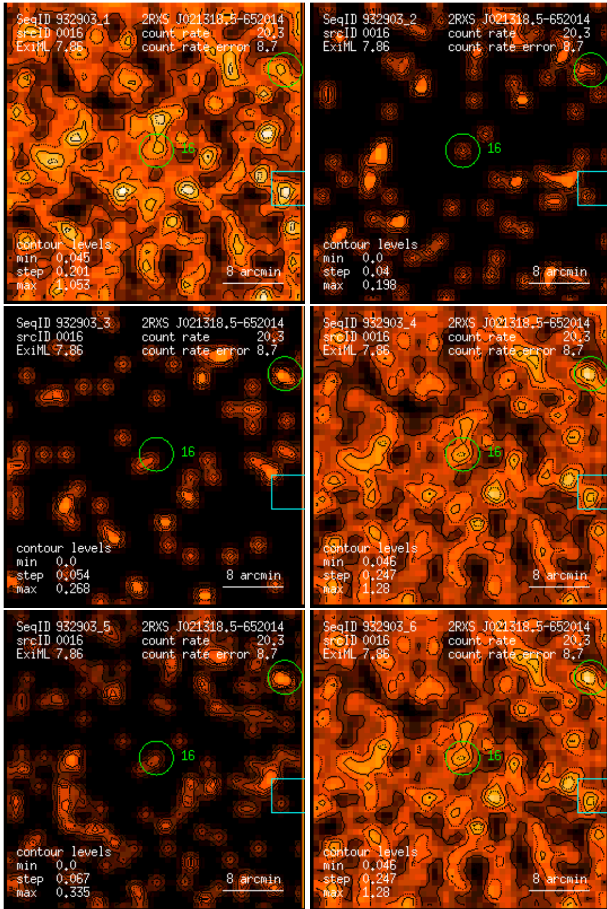
Figure 16: RASS 932903: detection 0016: band rate images, Gaussian filter: (1) PSPC channels 11 – 41, (2) 52 – 90, (3) 91 – 201, (4) 11 – 235, (5) 52 – 201, (6) 11 – 201. Broad band rates in counts/ks. Band rate contour levels in counts/ks/arcmin 2 .
