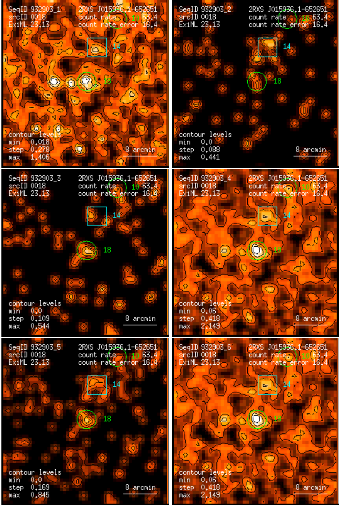
Figure 18: RASS 932903: detection 0018: band rate images, Gaussian filter: (1) PSPC channels 11 – 41, (2) 52 – 90, (3) 91 – 201, (4) 11 – 235, (5) 52 – 201, (6) 11 – 201. Broad band rates in counts/ks. Band rate contour levels in counts/ks/arcmin 2 .
