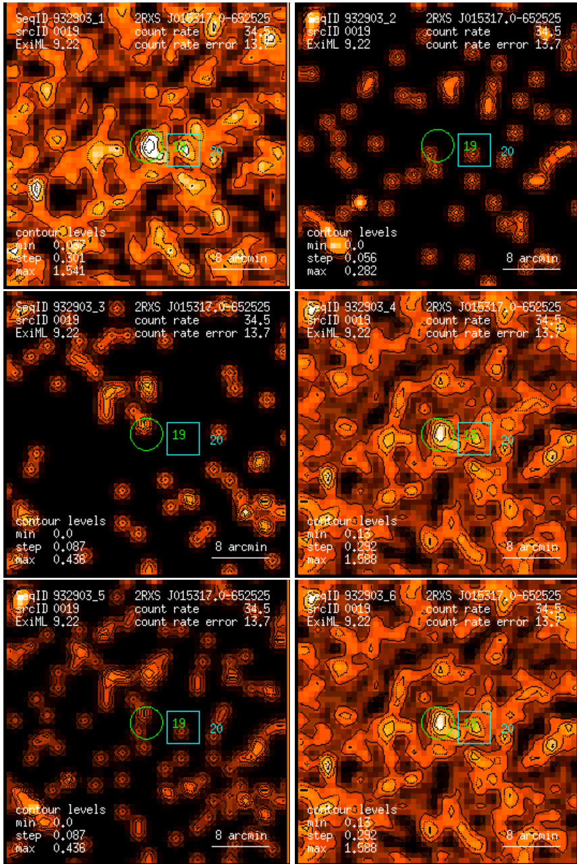
Figure 19: RASS 932903: detection 0019: band rate images, Gaussian filter: (1) PSPC channels 11 – 41, (2) 52 – 90, (3) 91 – 201, (4) 11 – 235, (5) 52 – 201, (6) 11 – 201. Broad band rates in counts/ks. Band rate contour levels in counts/ks/arcmin 2 .
