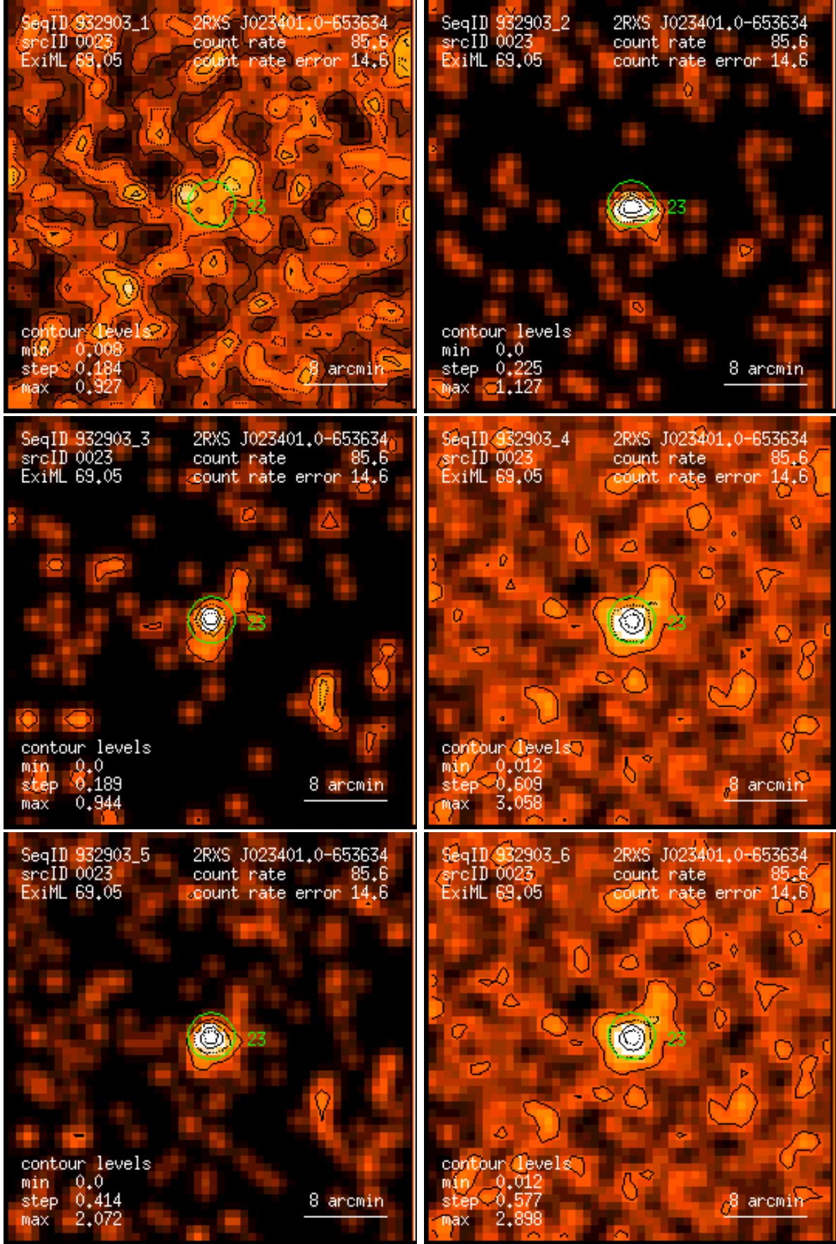
Figure 23: RASS 932903: detection 0023: band rate images, Gaussian filter: (1) PSPC channels 11 – 41, (2) 52 – 90, (3) 91 – 201, (4) 11 – 235, (5) 52 – 201, (6) 11 – 201. Broad band rates in counts/ks. Band rate contour levels in counts/ks/arcmin 2 .
