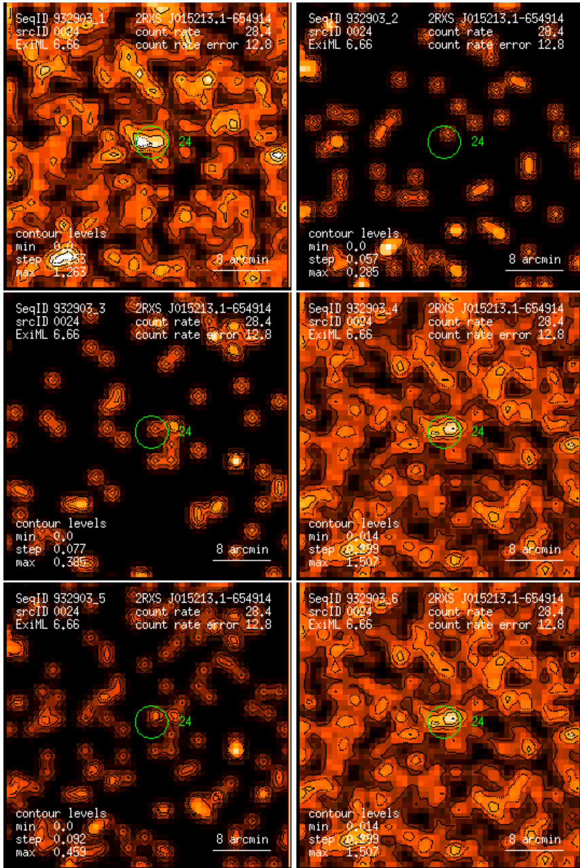
Figure 24: RASS 932903: detection 0024: band rate images, Gaussian filter: (1) PSPC channels 11 – 41, (2) 52 – 90, (3) 91 – 201, (4) 11 – 235, (5) 52 – 201, (6) 11 – 201. Broad band rates in counts/ks. Band rate contour levels in counts/ks/arcmin 2 .
