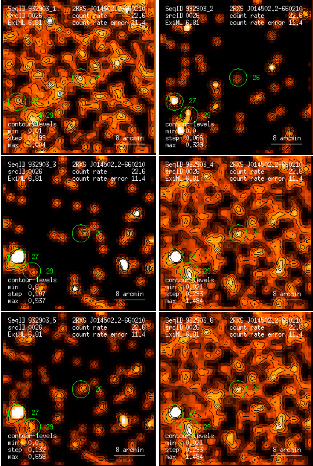
Figure 26: RASS 932903: detection 0026: band rate images, Gaussian filter: (1) PSPC channels 11 – 41, (2) 52 – 90, (3) 91 – 201, (4) 11 – 235, (5) 52 – 201, (6) 11 – 201. Broad band rates in counts/ks. Band rate contour levels in counts/ks/arcmin 2 .
