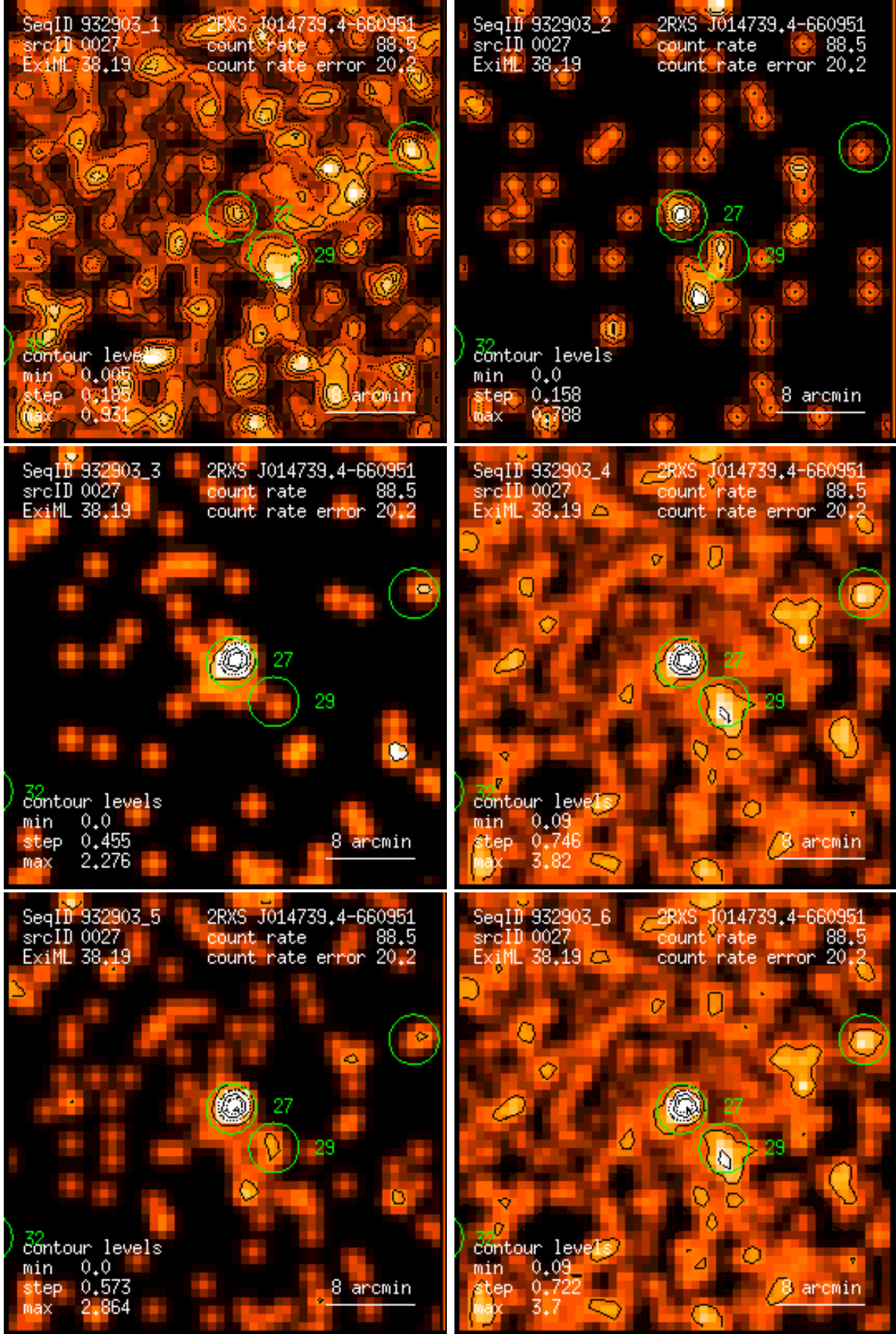
Figure 27: RASS 932903: detection 0027: band rate images, Gaussian filter: (1) PSPC channels 11 – 41, (2) 52 – 90, (3) 91 – 201, (4) 11 – 235, (5) 52 – 201, (6) 11 – 201. Broad band rates in counts/ks. Band rate contour levels in counts/ks/arcmin 2 .
