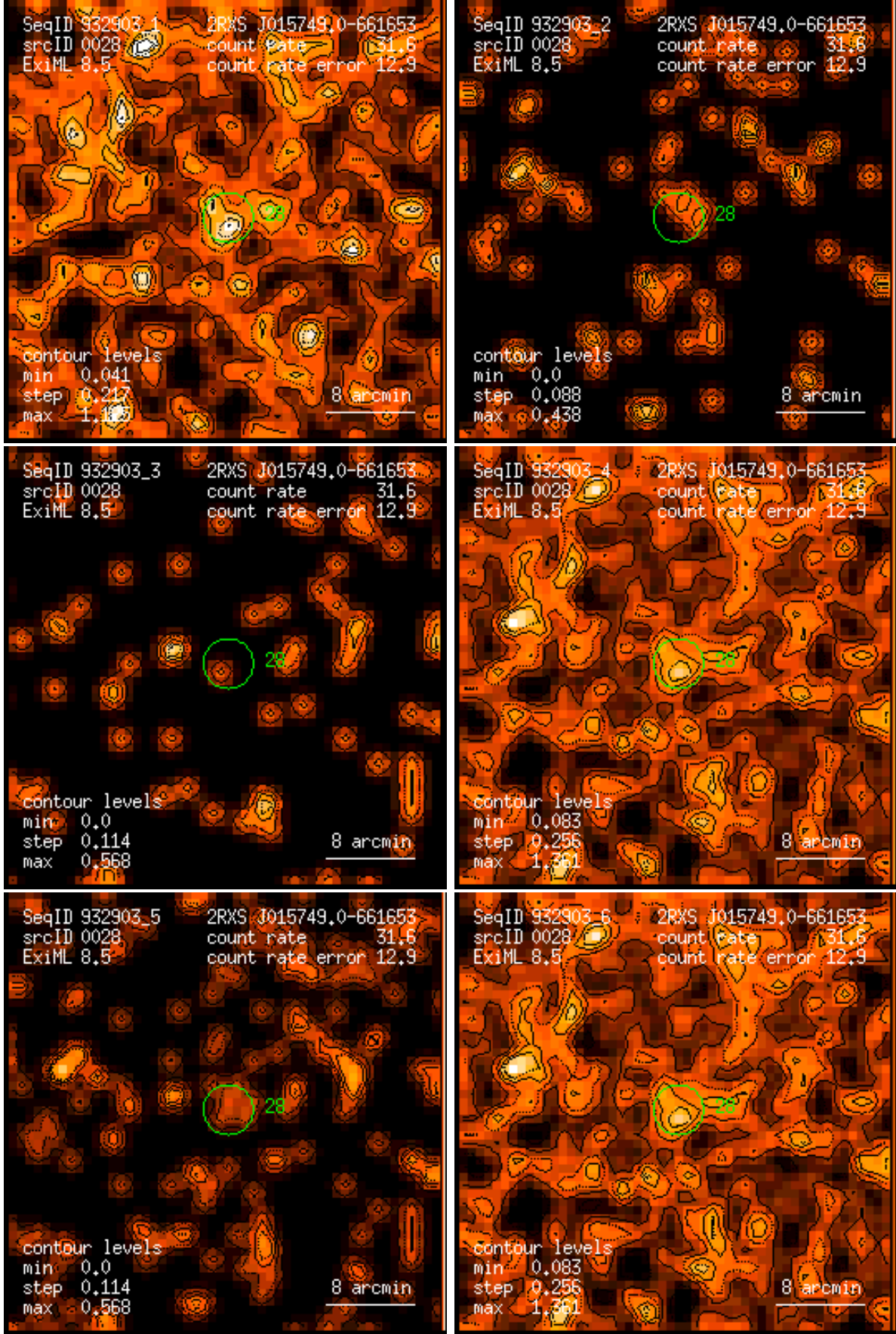
Figure 28: RASS 932903: detection 0028: band rate images, Gaussian filter: (1) PSPC channels 11 – 41, (2) 52 – 90, (3) 91 – 201, (4) 11 – 235, (5) 52 – 201, (6) 11 – 201. Broad band rates in counts/ks. Band rate contour levels in counts/ks/arcmin 2 .
