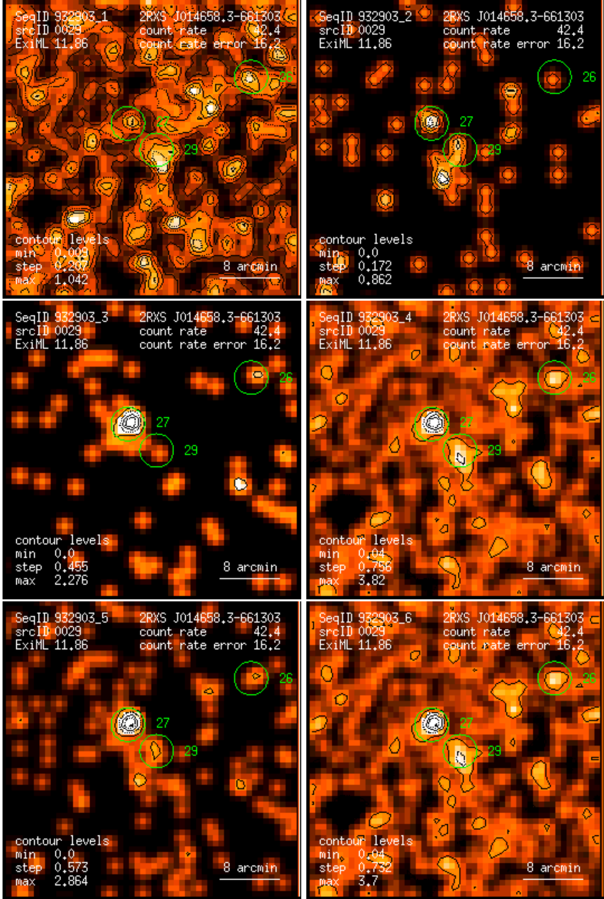
Figure 29: RASS 932903: detection 0029: band rate images, Gaussian filter: (1) PSPC channels 11 – 41, (2) 52 – 90, (3) 91 – 201, (4) 11 – 235, (5) 52 – 201, (6) 11 – 201. Broad band rates in counts/ks. Band rate contour levels in counts/ks/arcmin 2 .
