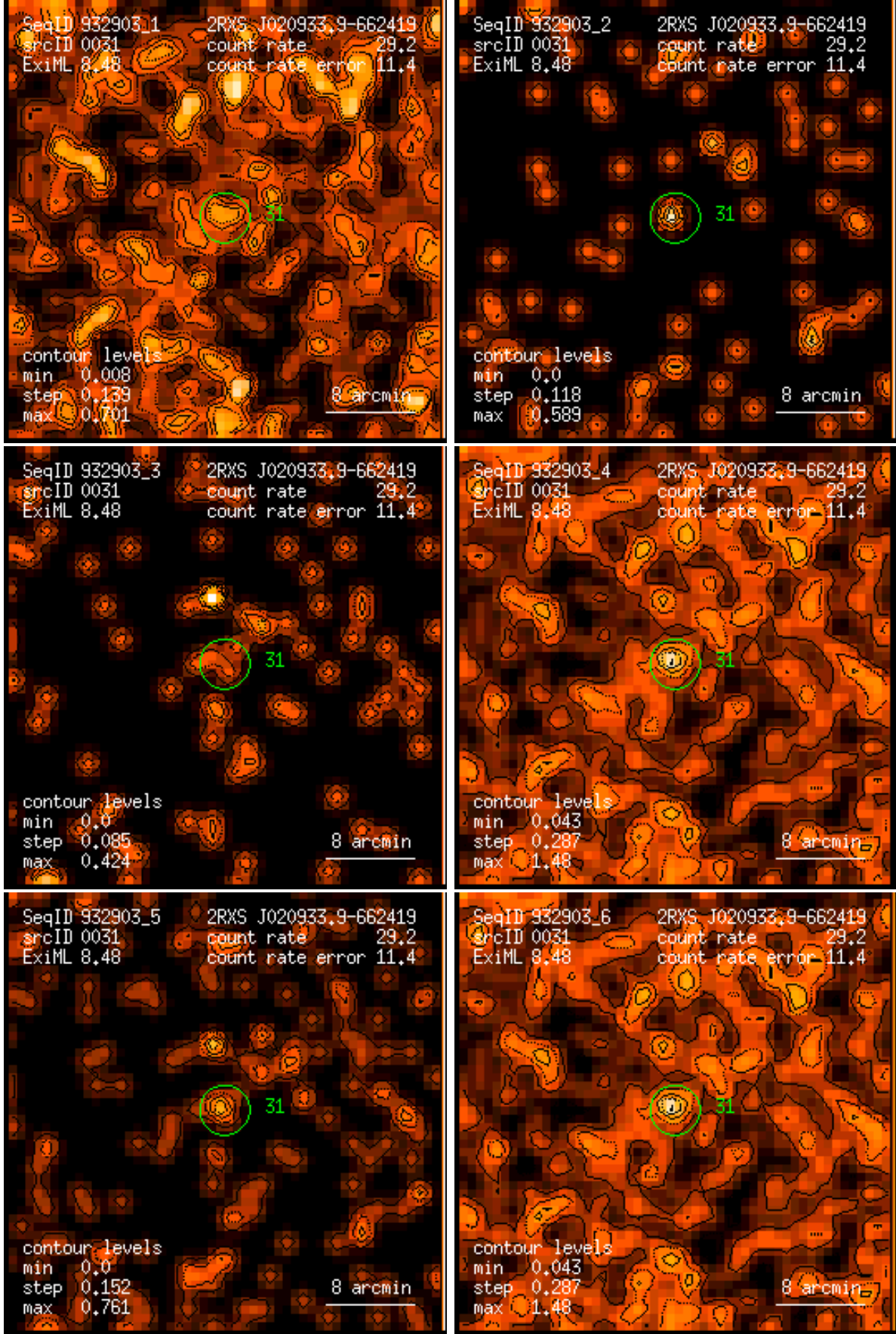
Figure 31: RASS 932903: detection 0031: band rate images, Gaussian filter: (1) PSPC channels 11 – 41, (2) 52 – 90, (3) 91 – 201, (4) 11 – 235, (5) 52 – 201, (6) 11 – 201. Broad band rates in counts/ks. Band rate contour levels in counts/ks/arcmin 2 .
