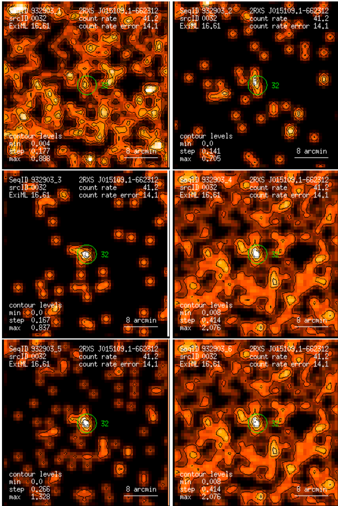
Figure 32: RASS 932903: detection 0032: band rate images, Gaussian filter: (1) PSPC channels 11 – 41, (2) 52 – 90, (3) 91 – 201, (4) 11 – 235, (5) 52 – 201, (6) 11 – 201. Broad band rates in counts/ks. Band rate contour levels in counts/ks/arcmin 2 .
