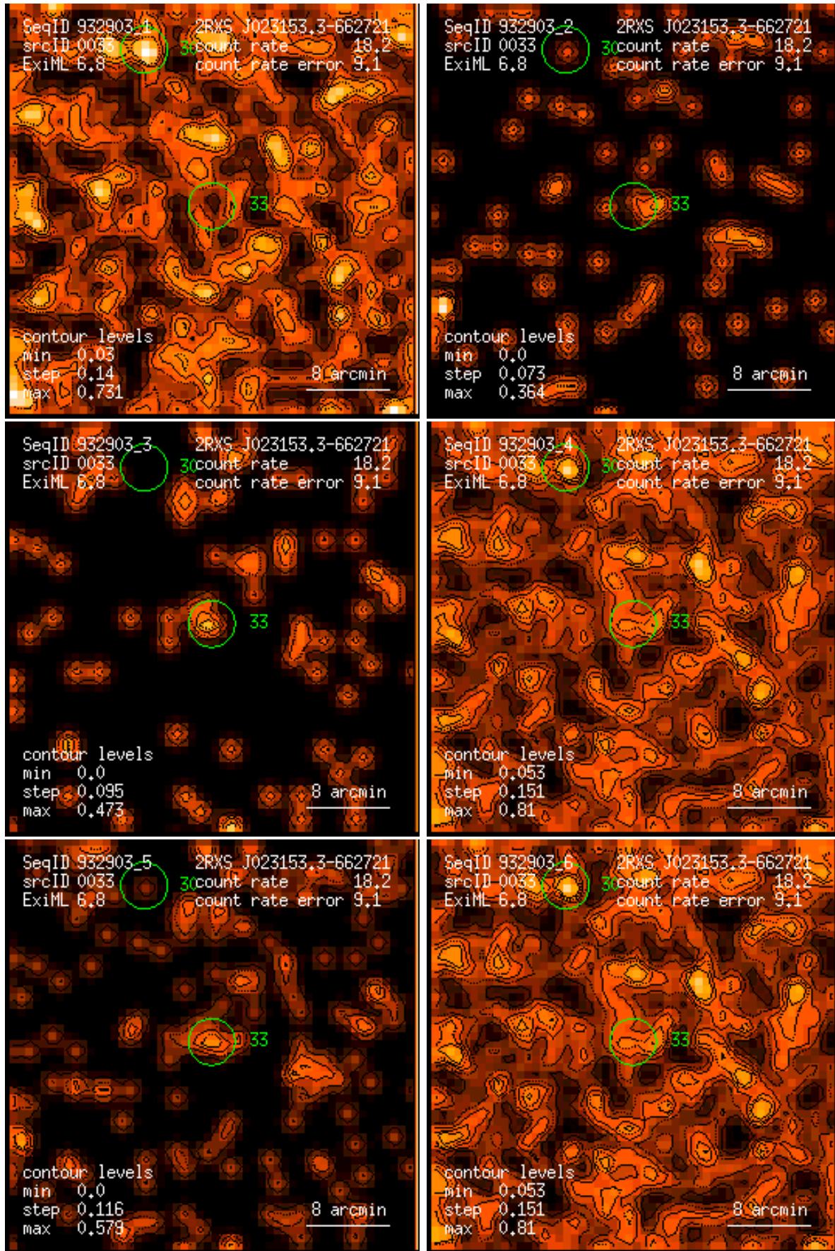
Figure 33: RASS 932903: detection 0033: band rate images, Gaussian filter: (1) PSPC channels 11 – 41, (2) 52 – 90, (3) 91 – 201, (4) 11 – 235, (5) 52 – 201, (6) 11 – 201. Broad band rates in counts/ks. Band rate contour levels in counts/ks/arcmin 2 .
