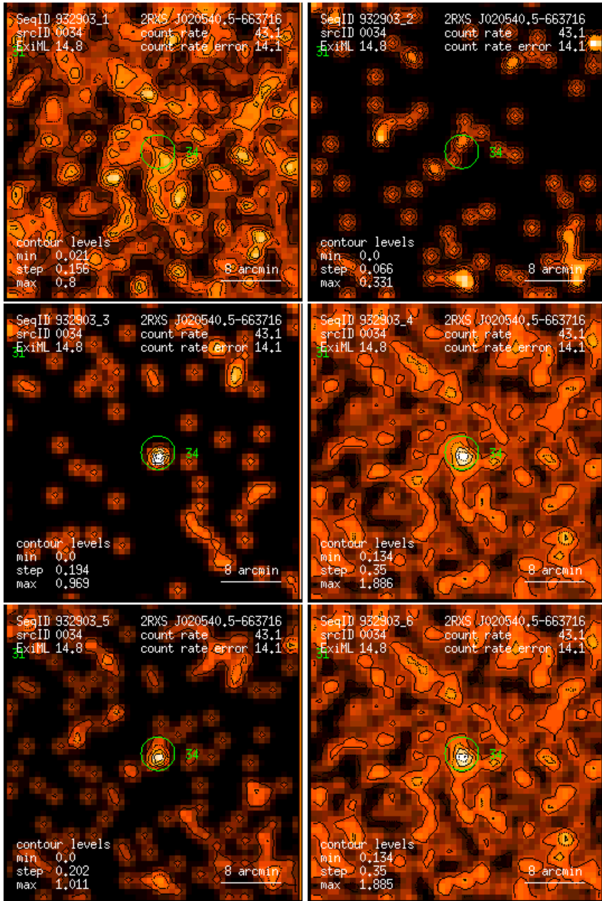
Figure 34: RASS 932903: detection 0034: band rate images, Gaussian filter: (1) PSPC channels 11 – 41, (2) 52 – 90, (3) 91 – 201, (4) 11 – 235, (5) 52 – 201, (6) 11 – 201. Broad band rates in counts/ks. Band rate contour levels in counts/ks/arcmin 2 .
