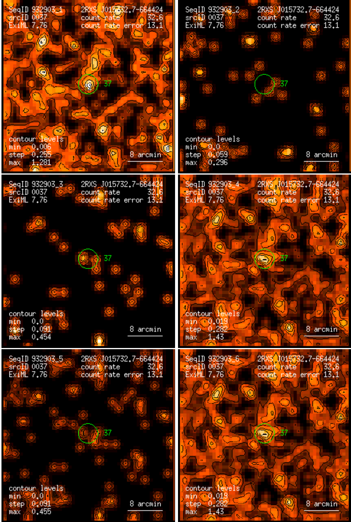
Figure 37: RASS 932903: detection 0037: band rate images, Gaussian filter: (1) PSPC channels 11 – 41, (2) 52 – 90, (3) 91 – 201, (4) 11 – 235, (5) 52 – 201, (6) 11 – 201. Broad band rates in counts/ks. Band rate contour levels in counts/ks/arcmin 2 .
