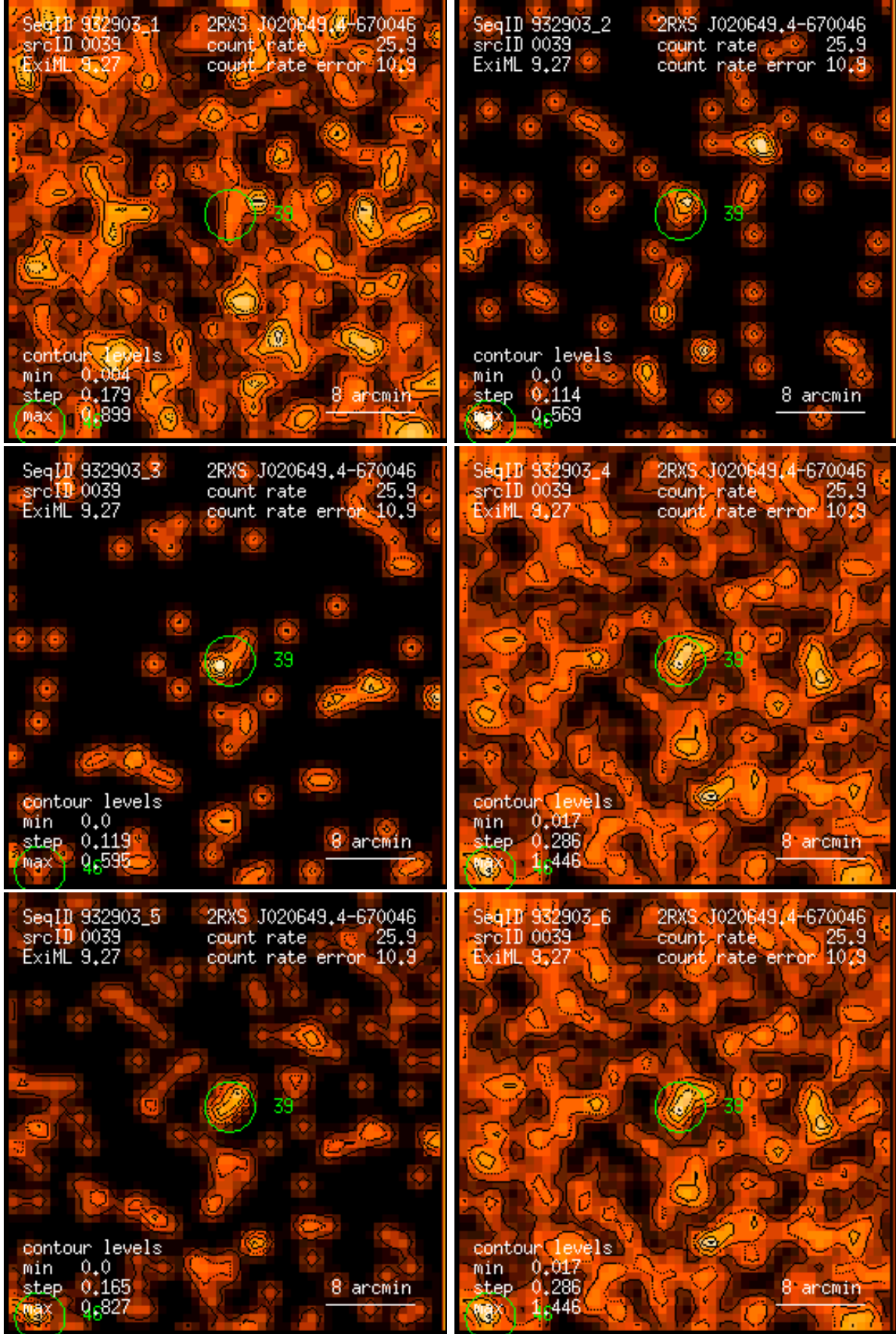
Figure 39: RASS 932903: detection 0039: band rate images, Gaussian filter: (1) PSPC channels 11 – 41, (2) 52 – 90, (3) 91 – 201, (4) 11 – 235, (5) 52 – 201, (6) 11 – 201. Broad band rates in counts/ks. Band rate contour levels in counts/ks/arcmin 2 .
