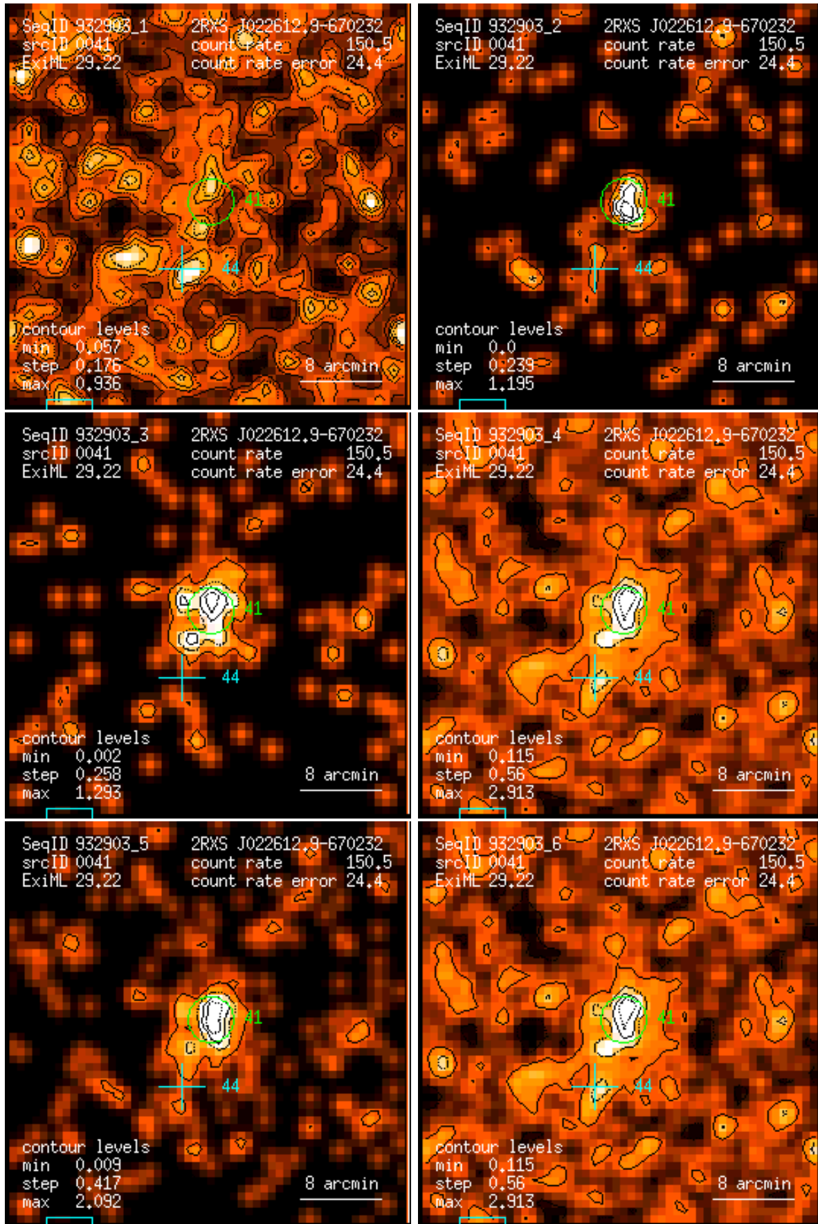
Figure 41: RASS 932903: detection 0041: band rate images, Gaussian filter: (1) PSPC channels 11 – 41, (2) 52 – 90, (3) 91 – 201, (4) 11 – 235, (5) 52 – 201, (6) 11 – 201. Broad band rates in counts/ks. Band rate contour levels in counts/ks/arcmin 2 .
