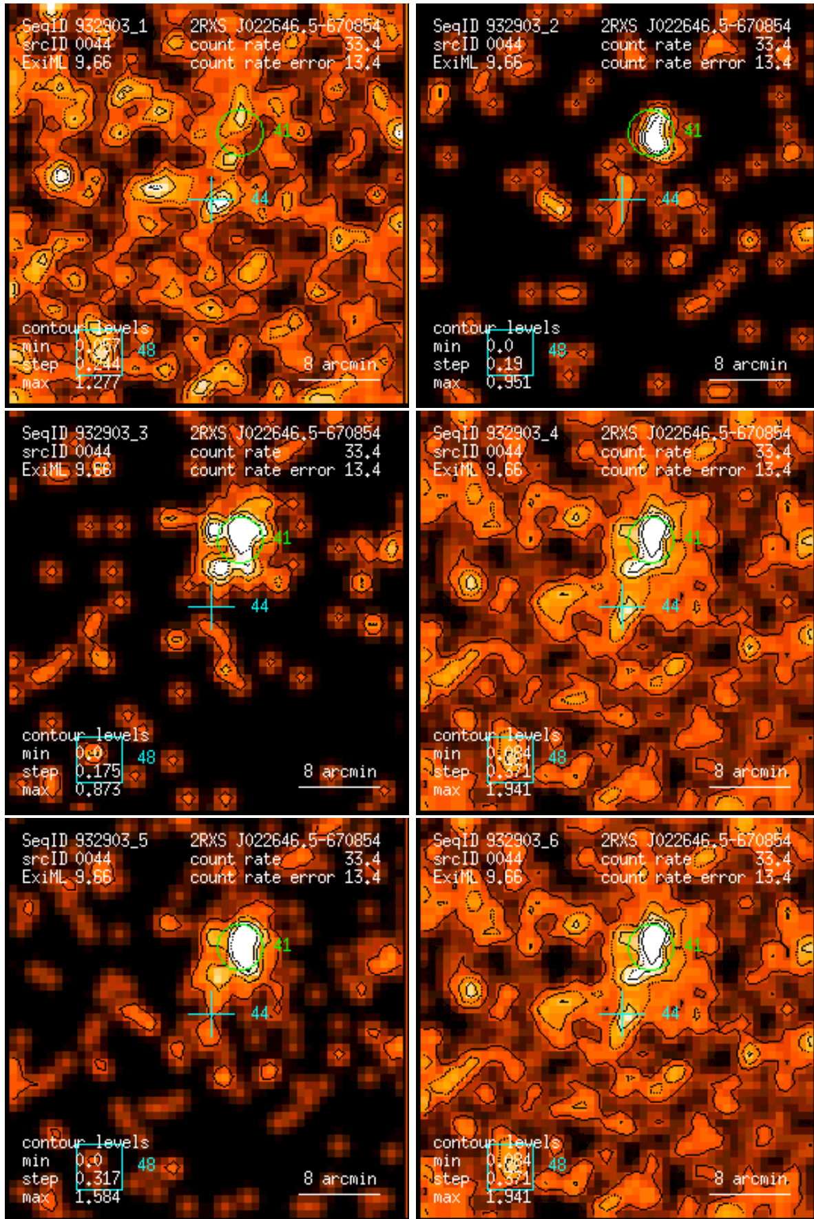
Figure 44: RASS 932903: detection 0044: band rate images, Gaussian filter: (1) PSPC channels 11 – 41, (2) 52 – 90, (3) 91 – 201, (4) 11 – 235, (5) 52 – 201, (6) 11 – 201. Broad band rates in counts/ks. Band rate contour levels in counts/ks/arcmin 2 .
