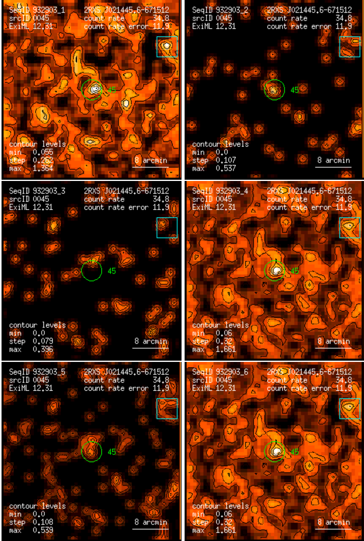
Figure 45: RASS 932903: detection 0045: band rate images, Gaussian filter: (1) PSPC channels 11 – 41, (2) 52 – 90, (3) 91 – 201, (4) 11 – 235, (5) 52 – 201, (6) 11 – 201. Broad band rates in counts/ks. Band rate contour levels in counts/ks/arcmin 2 .
