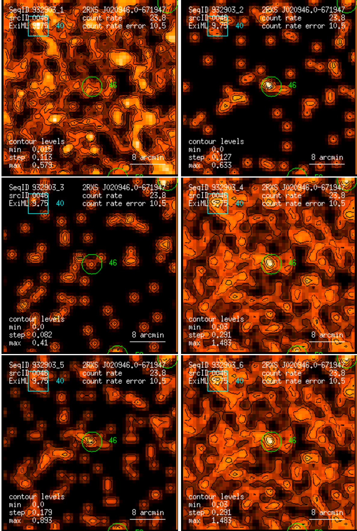
Figure 46: RASS 932903: detection 0046: band rate images, Gaussian filter: (1) PSPC channels 11 – 41, (2) 52 – 90, (3) 91 – 201, (4) 11 – 235, (5) 52 – 201, (6) 11 – 201. Broad band rates in counts/ks. Band rate contour levels in counts/ks/arcmin 2 .
