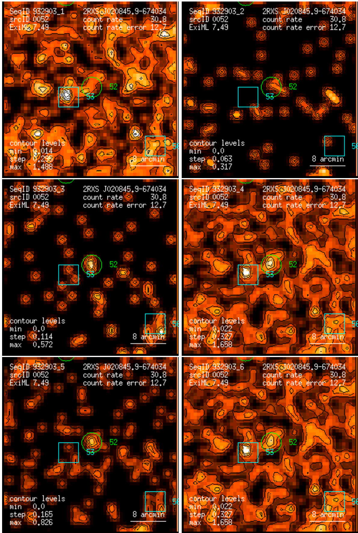
Figure 52: RASS 932903: detection 0052: band rate images, Gaussian filter: (1) PSPC channels 11 – 41, (2) 52 – 90, (3) 91 – 201, (4) 11 – 235, (5) 52 – 201, (6) 11 – 201. Broad band rates in counts/ks. Band rate contour levels in counts/ks/arcmin 2 .
