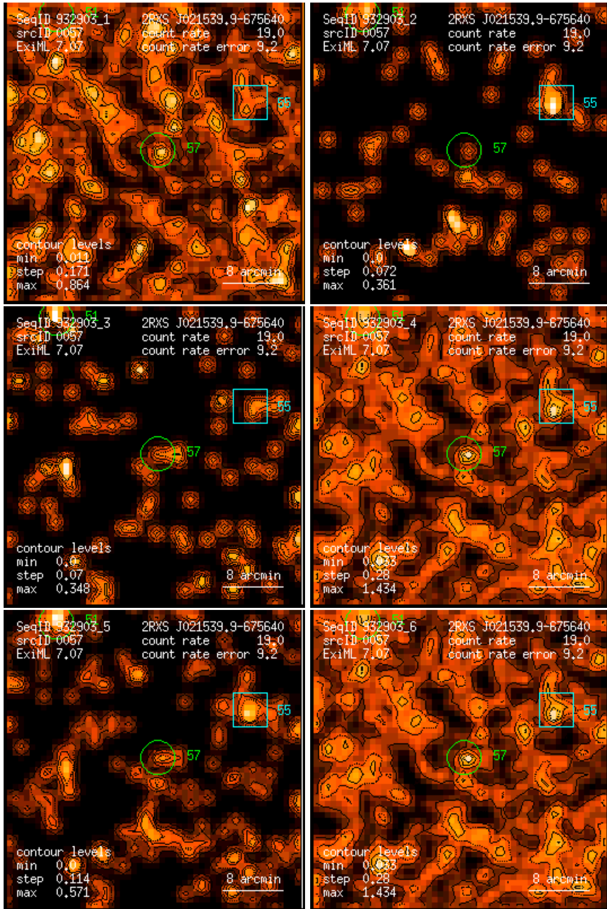
Figure 57: RASS 932903: detection 0057: band rate images, Gaussian filter: (1) PSPC channels 11 – 41, (2) 52 – 90, (3) 91 – 201, (4) 11 – 235, (5) 52 – 201, (6) 11 – 201. Broad band rates in counts/ks. Band rate contour levels in counts/ks/arcmin 2 .
