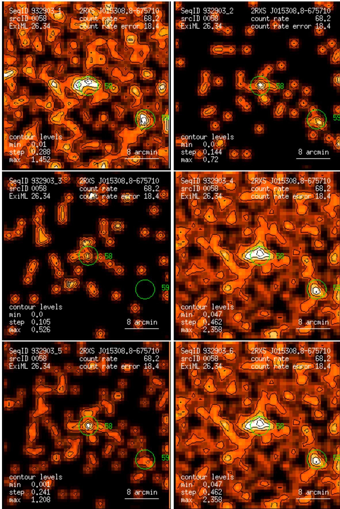
Figure 58: RASS 932903: detection 0058: band rate images, Gaussian filter: (1) PSPC channels 11 – 41, (2) 52 – 90, (3) 91 – 201, (4) 11 – 235, (5) 52 – 201, (6) 11 – 201. Broad band rates in counts/ks. Band rate contour levels in counts/ks/arcmin 2 .
