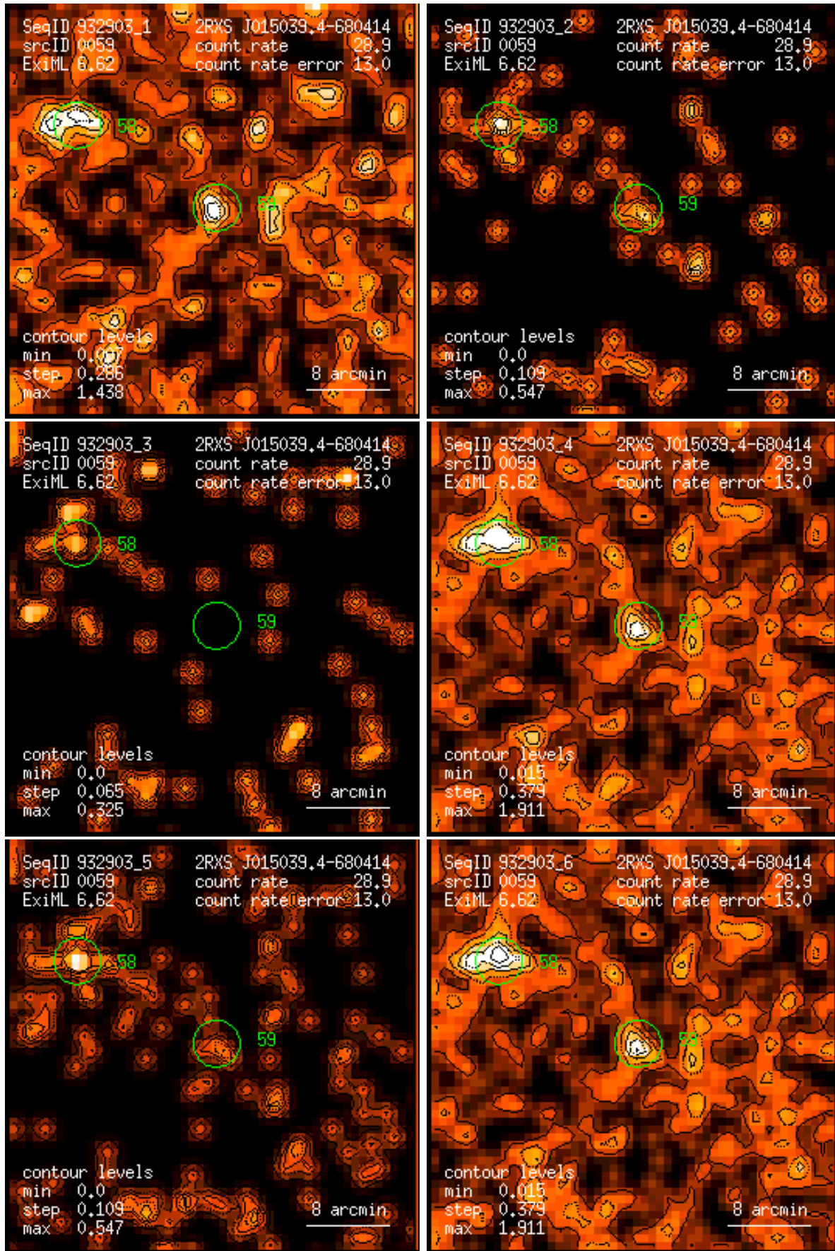
Figure 59: RASS 932903: detection 0059: band rate images, Gaussian filter: (1) PSPC channels 11 – 41, (2) 52 – 90, (3) 91 – 201, (4) 11 – 235, (5) 52 – 201, (6) 11 – 201. Broad band rates in counts/ks. Band rate contour levels in counts/ks/arcmin 2 .
