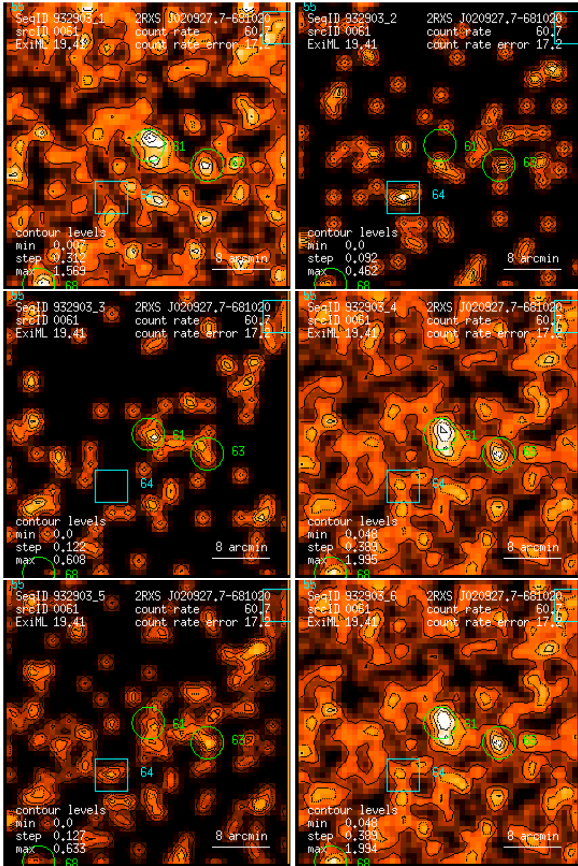
Figure 61: RASS 932903: detection 0061: band rate images, Gaussian filter: (1) PSPC channels 11 – 41, (2) 52 – 90, (3) 91 – 201, (4) 11 – 235, (5) 52 – 201, (6) 11 – 201. Broad band rates in counts/ks. Band rate contour levels in counts/ks/arcmin 2 .
