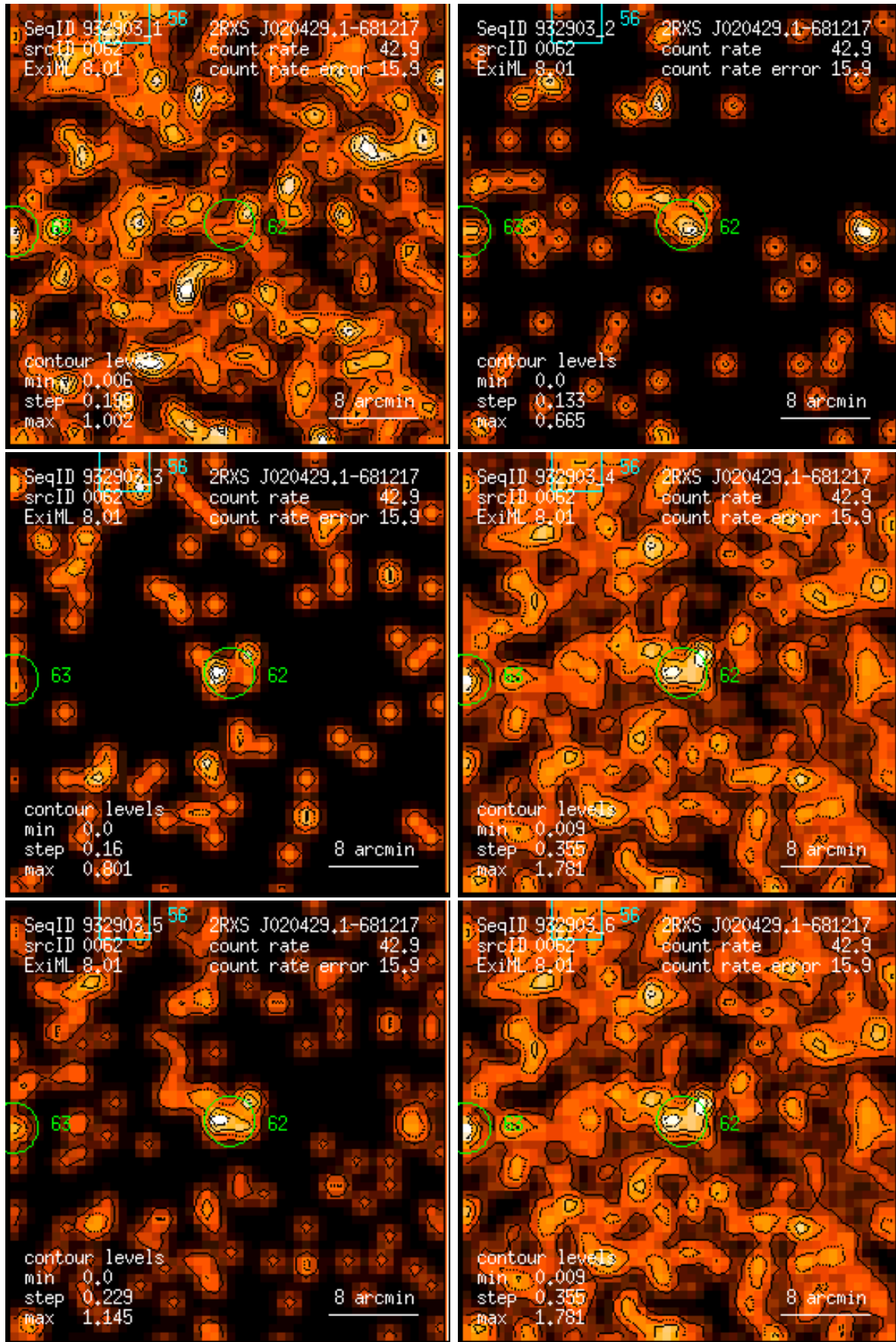
Figure 62: RASS 932903: detection 0062: band rate images, Gaussian filter: (1) PSPC channels 11 – 41, (2) 52 – 90, (3) 91 – 201, (4) 11 – 235, (5) 52 – 201, (6) 11 – 201. Broad band rates in counts/ks. Band rate contour levels in counts/ks/arcmin 2 .
