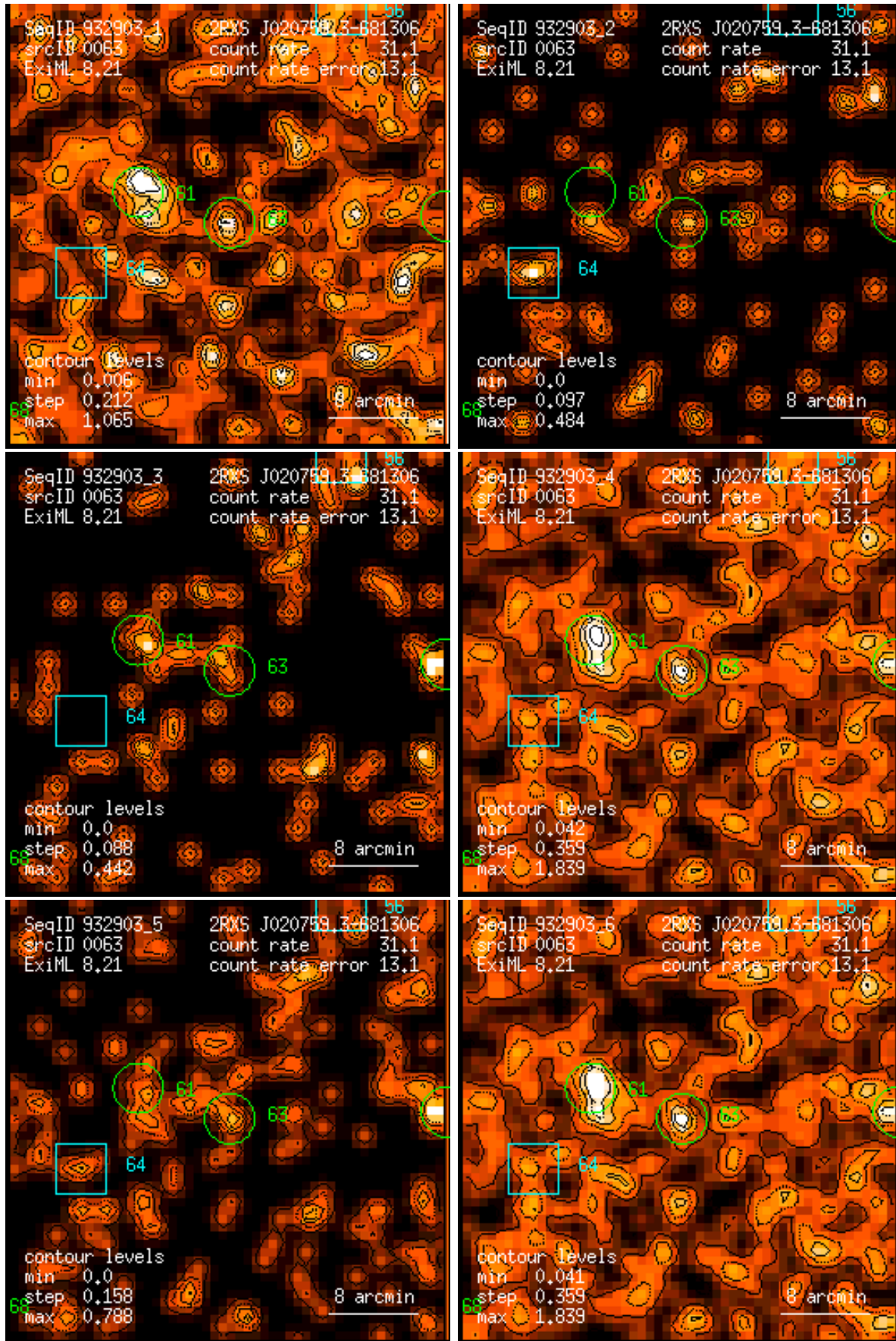
Figure 63: RASS 932903: detection 0063: band rate images, Gaussian filter: (1) PSPC channels 11 – 41, (2) 52 – 90, (3) 91 – 201, (4) 11 – 235, (5) 52 – 201, (6) 11 – 201. Broad band rates in counts/ks. Band rate contour levels in counts/ks/arcmin 2 .
