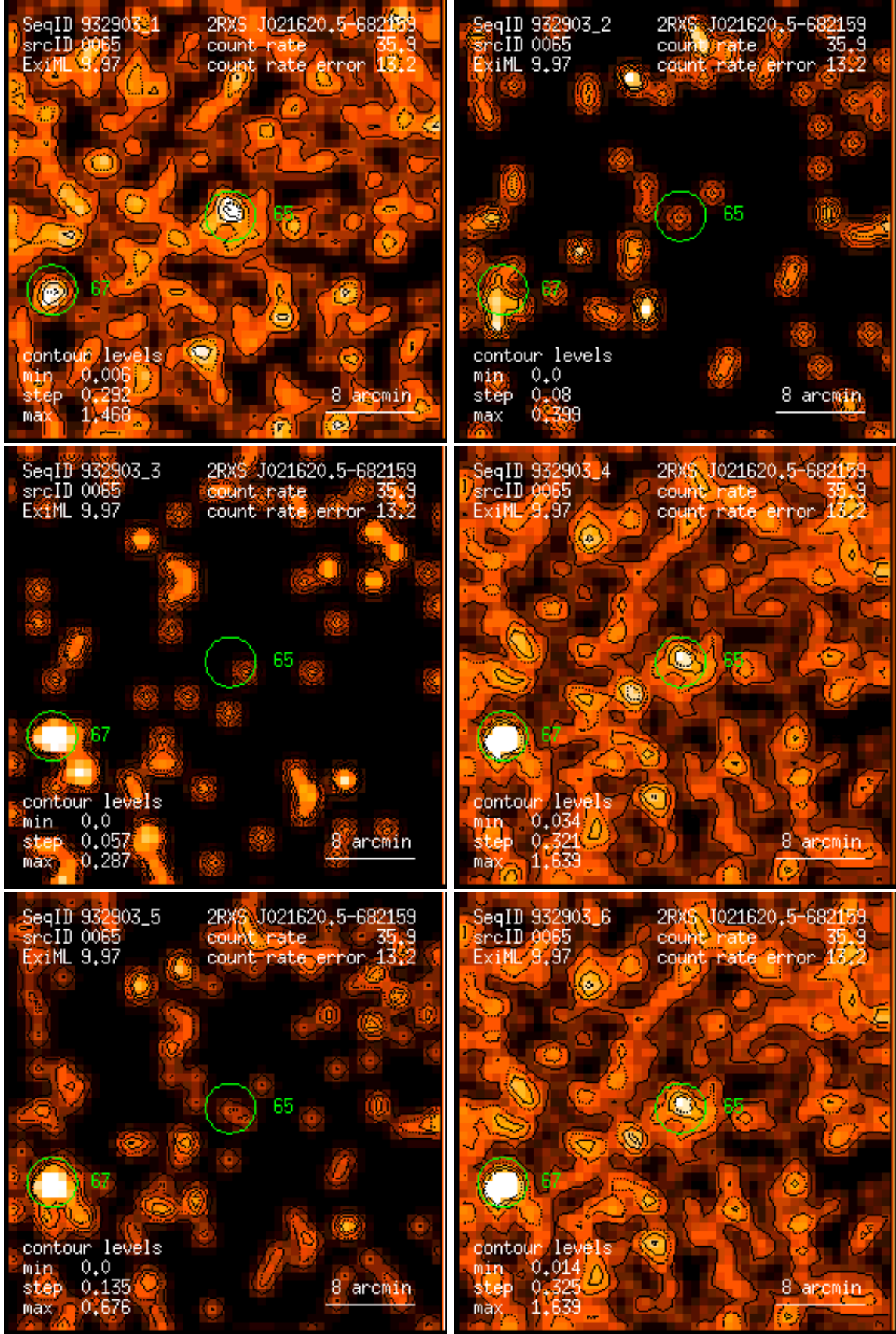
Figure 65: RASS 932903: detection 0065: band rate images, Gaussian filter: (1) PSPC channels 11 – 41, (2) 52 – 90, (3) 91 – 201, (4) 11 – 235, (5) 52 – 201, (6) 11 – 201. Broad band rates in counts/ks. Band rate contour levels in counts/ks/arcmin 2 .
