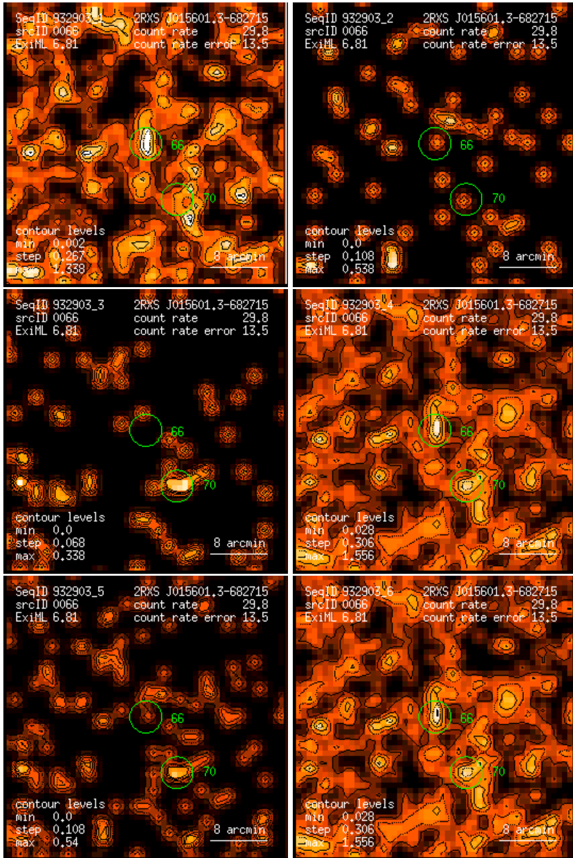
Figure 66: RASS 932903: detection 0066: band rate images, Gaussian filter: (1) PSPC channels 11 – 41, (2) 52 – 90, (3) 91 – 201, (4) 11 – 235, (5) 52 – 201, (6) 11 – 201. Broad band rates in counts/ks. Band rate contour levels in counts/ks/arcmin 2 .
