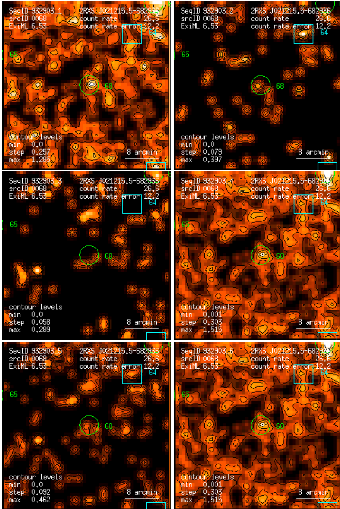
Figure 68: RASS 932903: detection 0068: band rate images, Gaussian filter: (1) PSPC channels 11 – 41, (2) 52 – 90, (3) 91 – 201, (4) 11 – 235, (5) 52 – 201, (6) 11 – 201. Broad band rates in counts/ks. Band rate contour levels in counts/ks/arcmin 2 .
