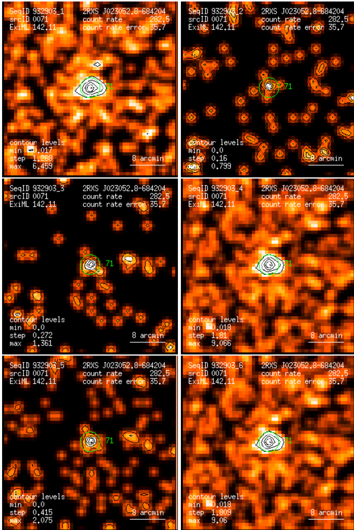
Figure 71: RASS 932903: detection 0071: band rate images, Gaussian filter: (1) PSPC channels 11 – 41, (2) 52 – 90, (3) 91 – 201, (4) 11 – 235, (5) 52 – 201, (6) 11 – 201. Broad band rates in counts/ks. Band rate contour levels in counts/ks/arcmin 2 .
