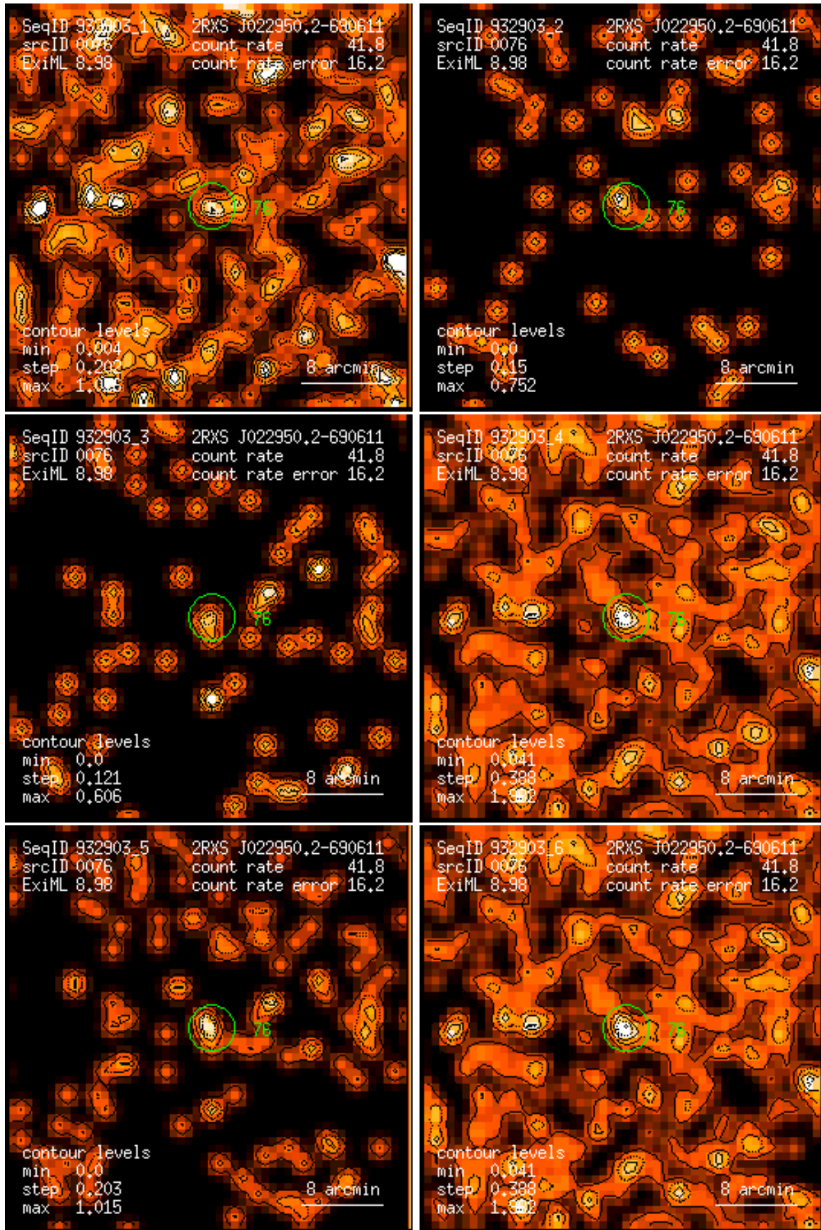
Figure 76: RASS 932903: detection 0076: band rate images, Gaussian filter: (1) PSPC channels 11 – 41, (2) 52 – 90, (3) 91 – 201, (4) 11 – 235, (5) 52 – 201, (6) 11 – 201. Broad band rates in counts/ks. Band rate contour levels in counts/ks/arcmin 2 .
