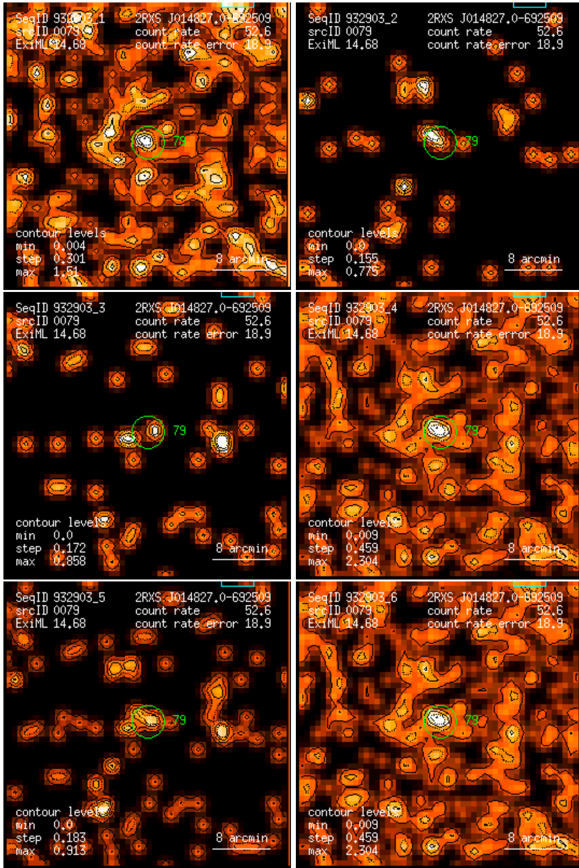
Figure 79: RASS 932903: detection 0079: band rate images, Gaussian filter: (1) PSPC channels 11 – 41, (2) 52 – 90, (3) 91 – 201, (4) 11 – 235, (5) 52 – 201, (6) 11 – 201. Broad band rates in counts/ks. Band rate contour levels in counts/ks/arcmin 2 .
