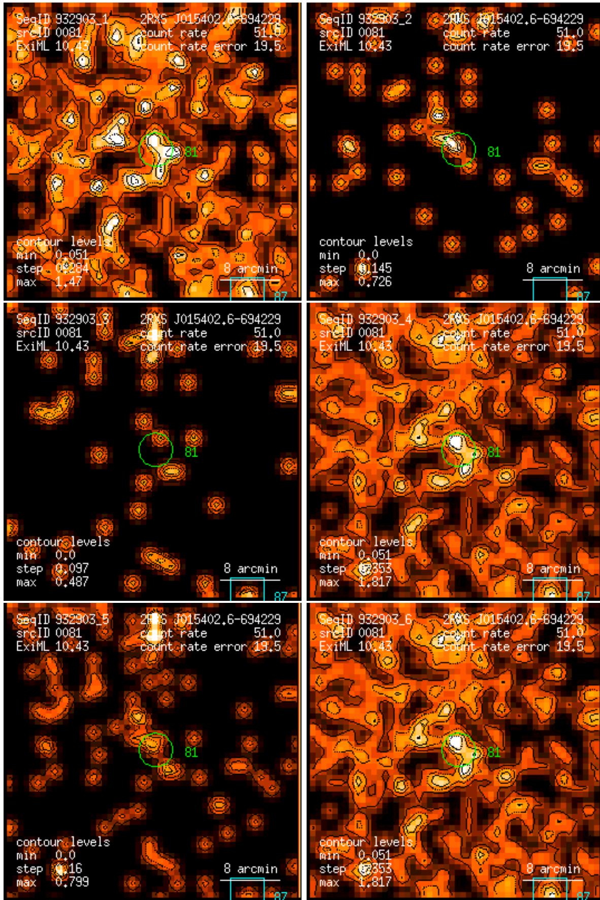
Figure 81: RASS 932903: detection 0081: band rate images, Gaussian filter: (1) PSPC channels 11 – 41, (2) 52 – 90, (3) 91 – 201, (4) 11 – 235, (5) 52 – 201, (6) 11 – 201. Broad band rates in counts/ks. Band rate contour levels in counts/ks/arcmin 2 .
