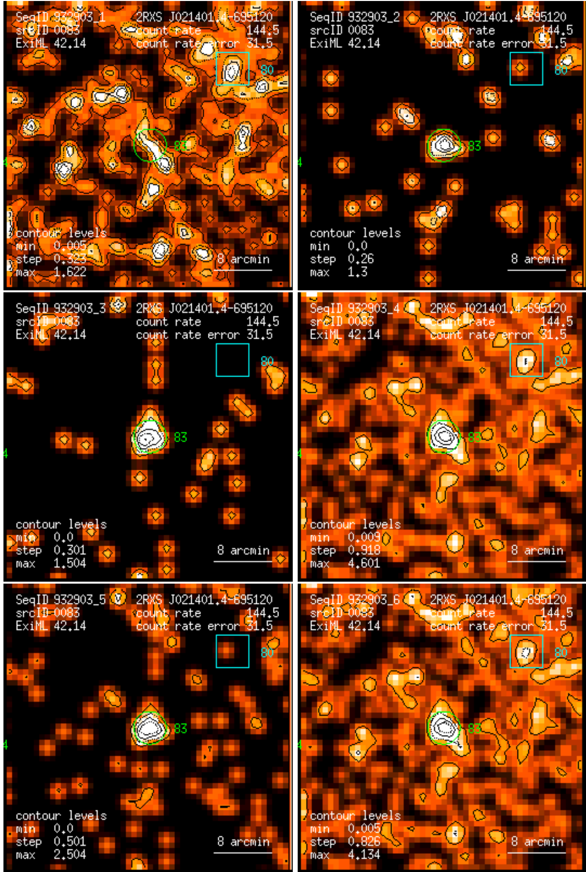
Figure 83: RASS 932903: detection 0083: band rate images, Gaussian filter: (1) PSPC channels 11 – 41, (2) 52 – 90, (3) 91 – 201, (4) 11 – 235, (5) 52 – 201, (6) 11 – 201. Broad band rates in counts/ks. Band rate contour levels in counts/ks/arcmin 2 .
